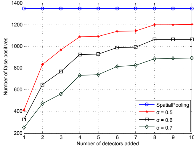
Figure 4.8. Number of false positives as a function of the number of detectors added and the threshold \sigma (results on INRIA Person dataset). The number of false positives obtained by the det_{root} alone (without our method) is shown as line because it is constant.
