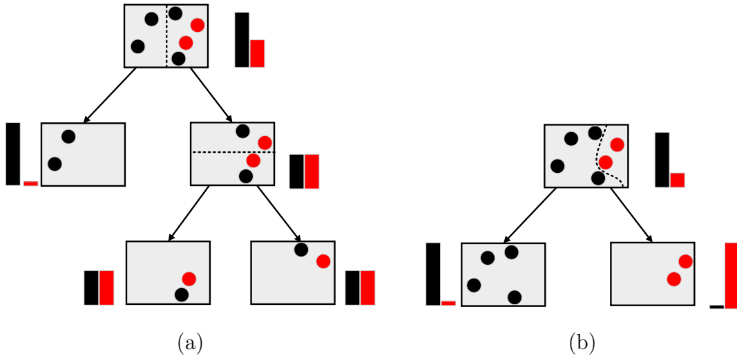
Figure 3.2. Decision tree split types (the bars represent the information gain). (a) Orthogonal split, tree with depth 2. (b) Oblique split, tree with depth 1.
