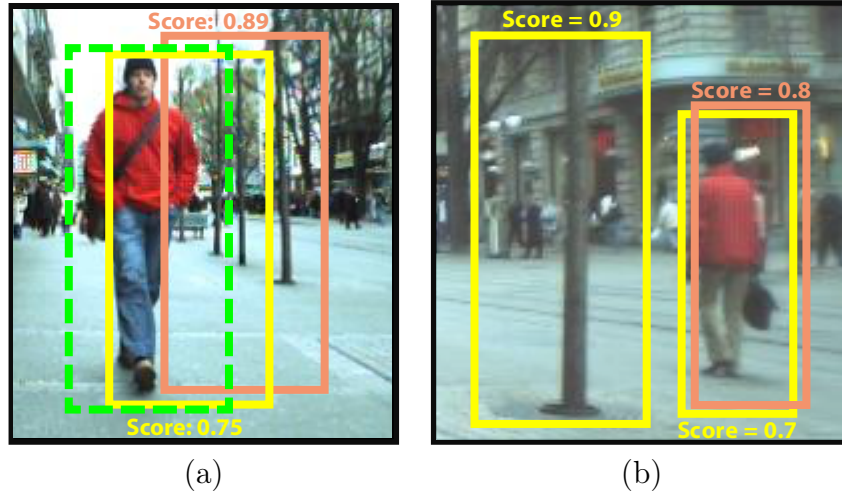
Figure 3.7. Different aspects between our proposed Spatial Consensus algorithm and the weighted-NMS [Jiang and Ma, 2015]. Yellow and orange boxes indicate the detection coming from det_{root} and det_j , respectively, and the dashed green box shows the ground-truth annotation. (a) Our Spatial Consensus algorithm will maintain the yellow box (true positive), since this window belongs to det_{root} , while the weighted-NMS will maintain the orange box (false positive) because it is the window with higher score, leading to higher miss rate and reduced recall; (b) The SC algorithm will remove the false positive in yellow since it has no spatial support of other detectors, while the weighted-NMS will keep this false positive window due to its high score (best visualized in color).
