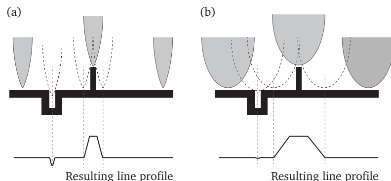
FIGURE 2.11: Illustration depicting the impact of a tip's apex dimension on the spatial resolution achieved. (a) A sharp tip traversing a sample and the obtained line profile. (b) The same as (a), but with a larger tip.
