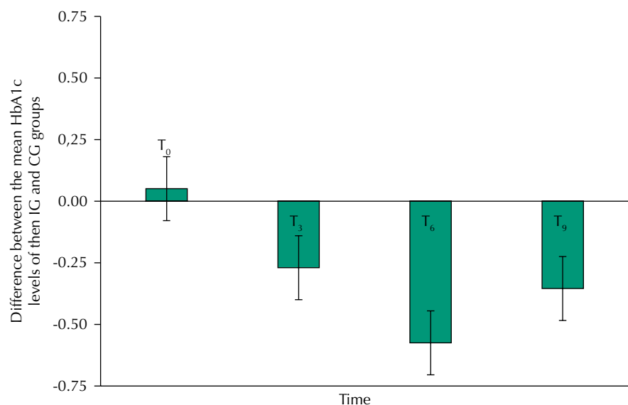
Figure 2. Average difference in HbA1c levels of the two groups over time: intervention group (IG) minus control group (CG). The intervals in the middle of the bars represent the 95% confidence intervals.
