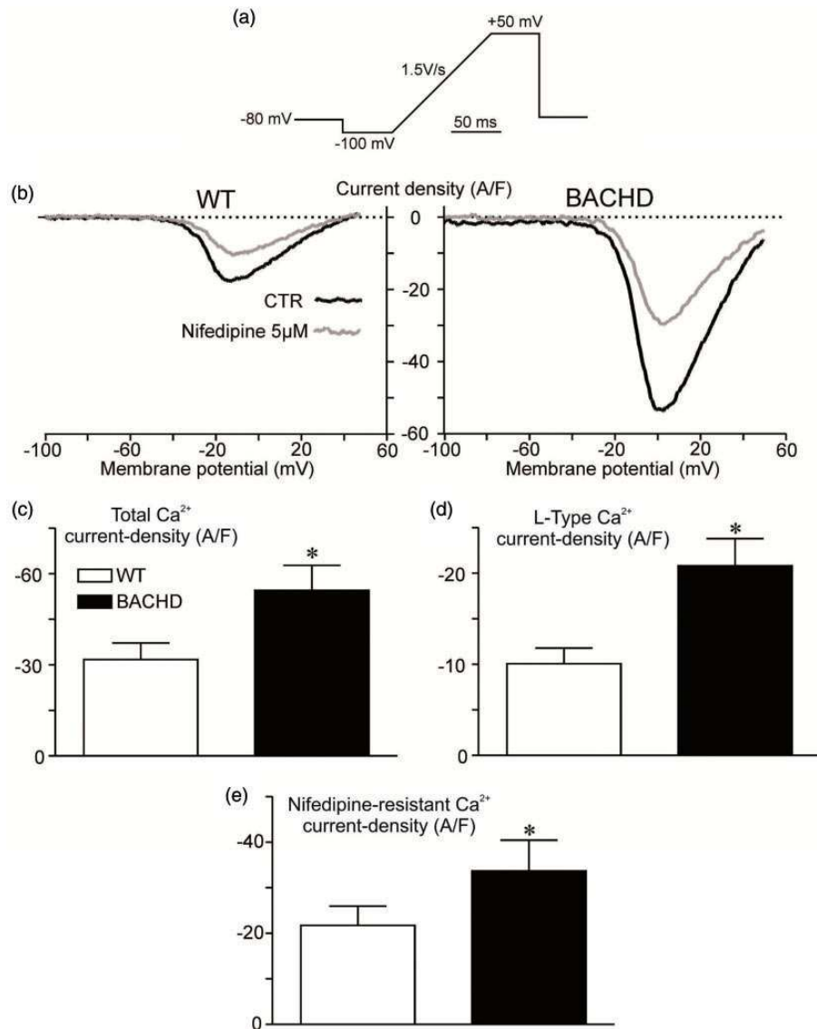
Figure 3. L-type Ca 2+ currents are increased in BACHD cortical neurons. (a) Voltage-clamp ramp protocol used to record I Ca currents. (b) Representative records of the Ca 2+ current–voltage relationship from WT (left panel) and BACHD (right panel) in the absence (black) or after exposure to nifedipine 5 μM (gray). (c) Graphs show peak total Ca 2+ current-density and (d) L-type Ca 2+ current-density from WT and BACHD mice. (e) Graphs show peak total Ca 2+ current-density after exposure to nifedipine 5 μM from WT (n = 8) and BACHD (n = 7) mice. *indicate significant differences as compared with matched WT (p < .05).
