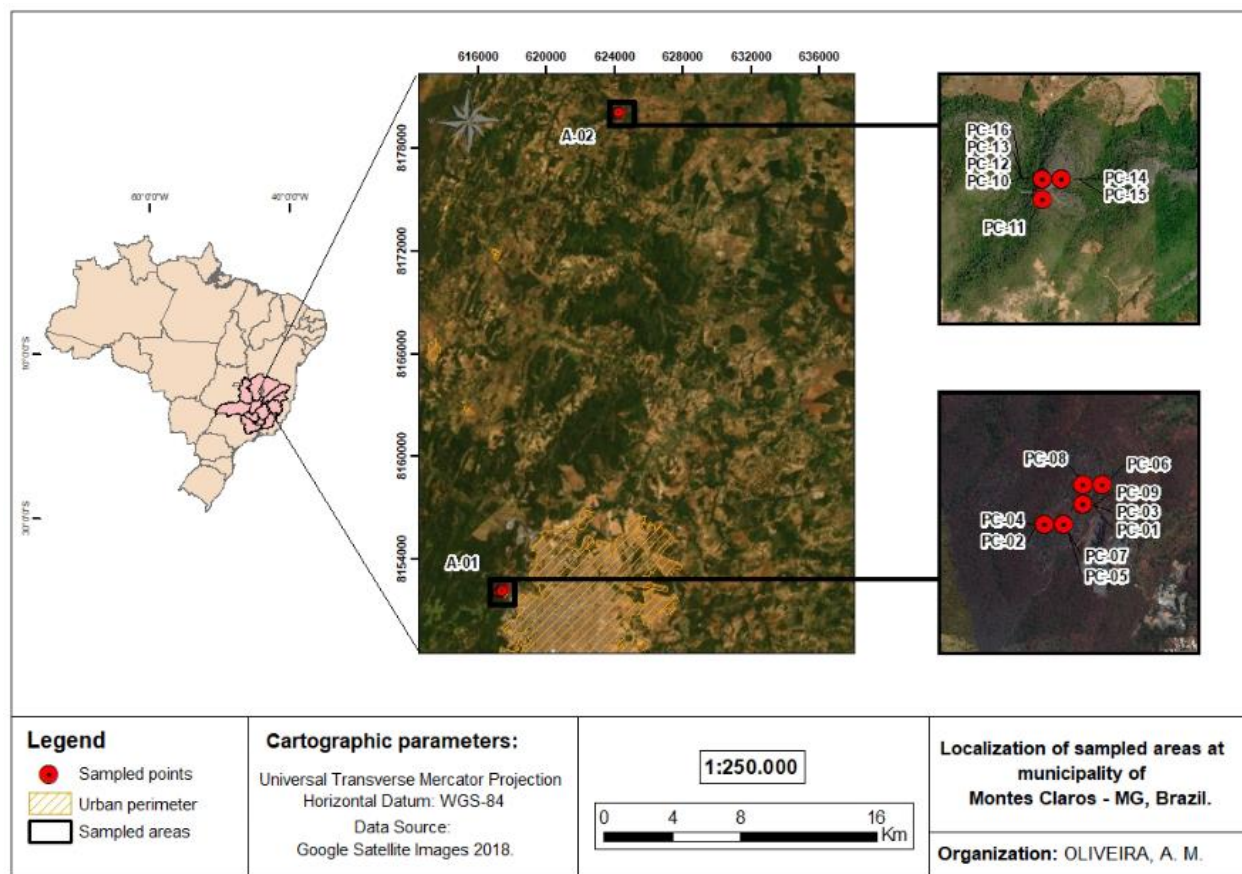
Figure 1 - Location of the studied areas and sampled points. Oliveira et al. (2023).
