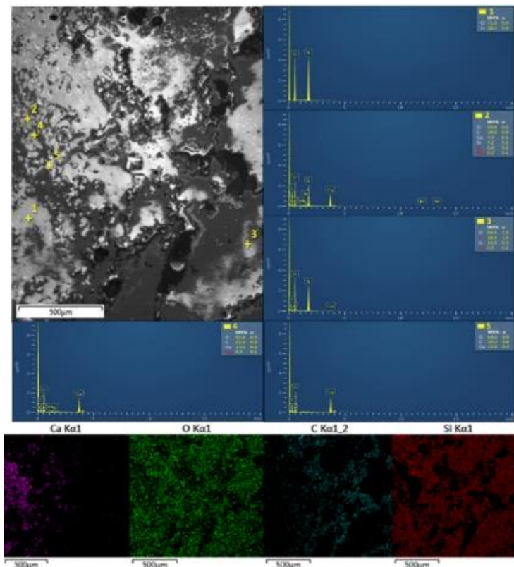
Figure 8 - Microchemical maps of the point P14 with backscattered electron images of the elements Ca, O, C, and Si obtained by EDS probe. The colored areas show the presence of the chemical element highlighted in the center of each image. Oliveira et al. (2023).
