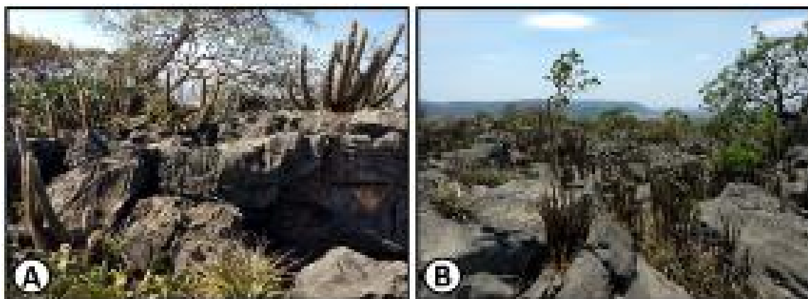
Figure 2 - Limestone outcrops and Karren formation, Montes Claros - MG, Brazil. Note: A) Area 01: Highlight for the Karren; B) Area 02: Landscape overview. Oliveira et al. (2023).
