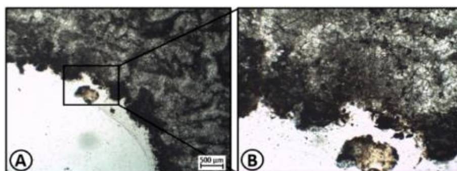
Figure 5 - Fragments of heavily altered rock, point P10. Note: A) Rock fragments; B) Detail of image A. Oliveira et al. (2023).
