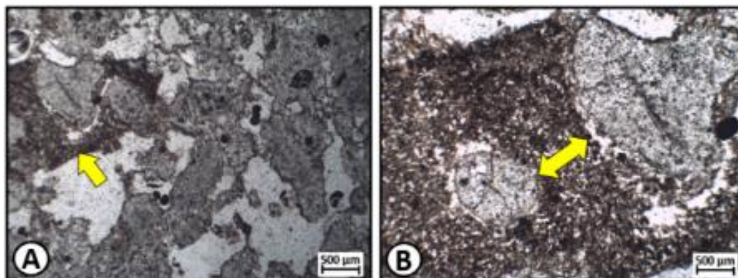
Figure 6 - Filling of pores by organic matter, point P14. Note: A) Irregular pores occupied by organic matter; B) Isolated rock fragments. Oliveira et al. (2023).
