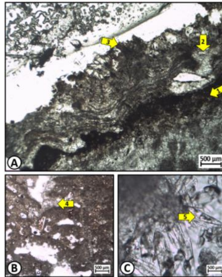
Figure 7 – Rodent/marsupial colonization. A and B: point 01; C: point 02. Note: Arrows indicate each stage of biokarstification; A1) Acidification; A2) Precipitation; A3) Discoloration; B4) precipitation; C5) Needle-fiber calcite. Oliveira et al. (2023).
