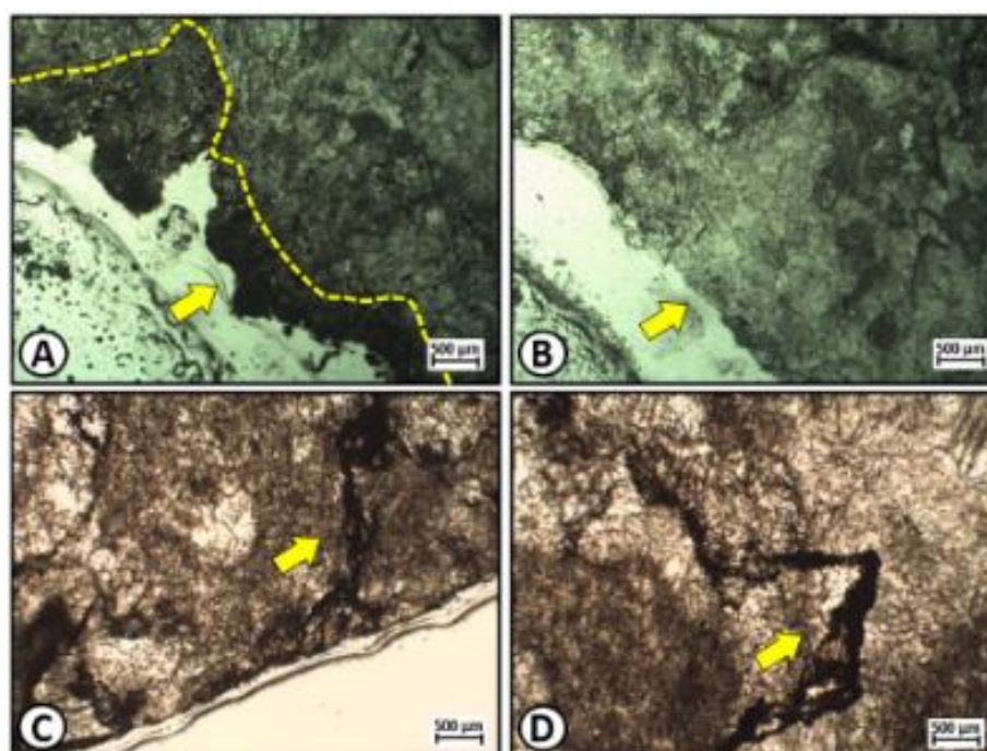
Figure 4 - Colonization areas with cyanobacteria, point P04. Note: A) With carapace; B) Without shell; C and D) Fractures with organic material. Oliveira et al. (2023).
