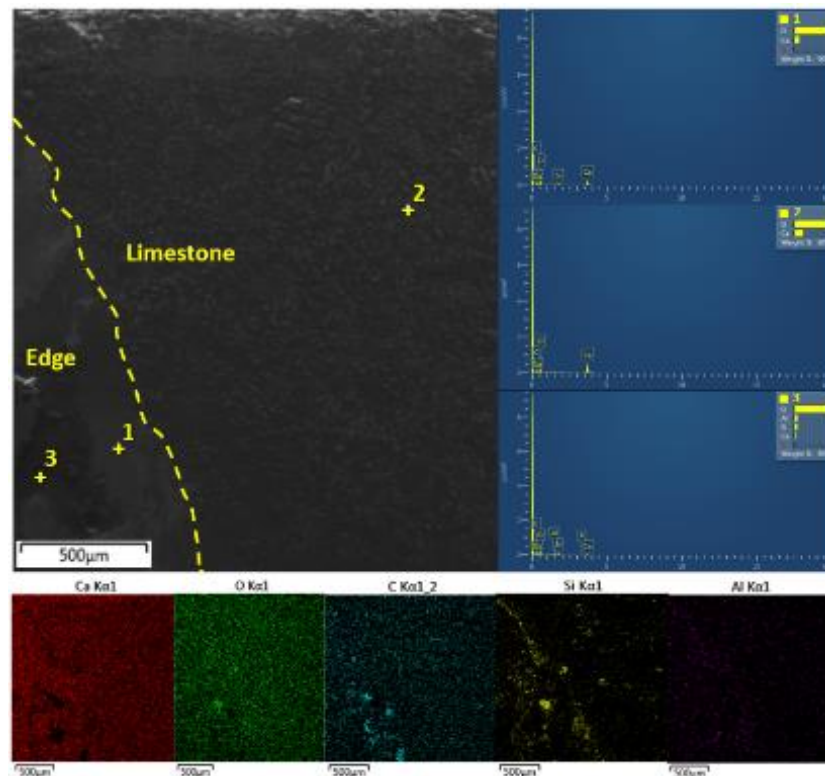
Figure 10 - Microchemical maps of point P01 with backscattered electron images of the elements Ca, O, C, Si, and Al obtained by EDS probe. The colored areas show the presence of the chemical element highlighted in the center of each image. Oliveira et al. (2023).
