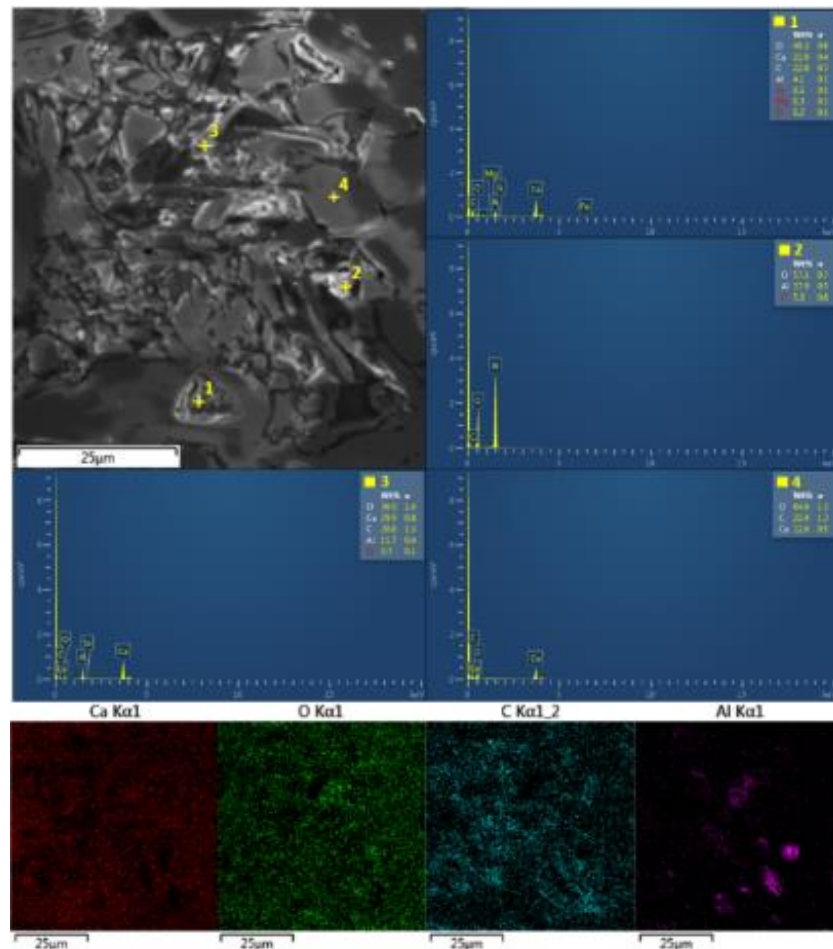
Figure 9 - Microchemical maps of the P02 point with backscattered electron images of the elements Ca, O, C, and Al obtained by EDS probe. The colored areas show the presence of the chemical element highlighted in the center of each image. Oliveira et al. (2023).
