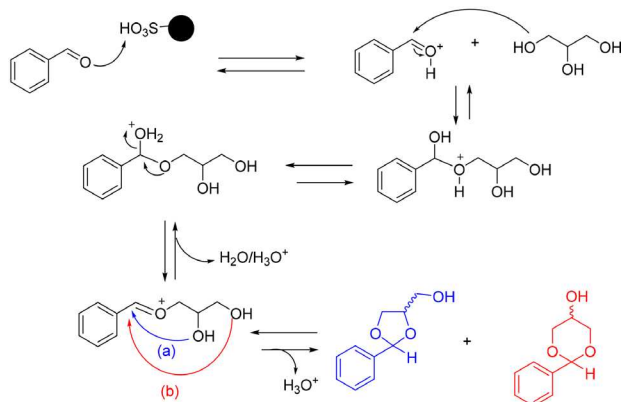
Figure 8. A proposed mechanism for obtaining five-membered (a) and six-membered (b) acetals from the reaction between benzaldehyde and glycerol.
