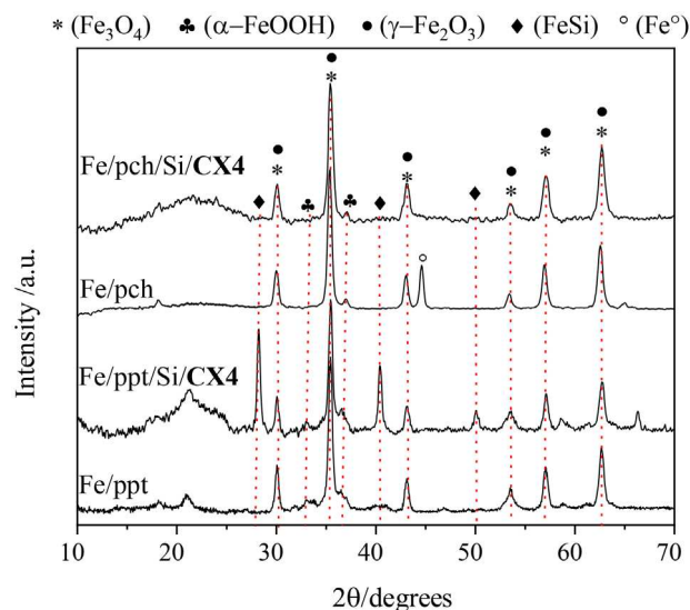
Figure 4. Powder XRD pattern of the iron oxides prepared by different methodologies and after the silanization/CX4 reactions.
