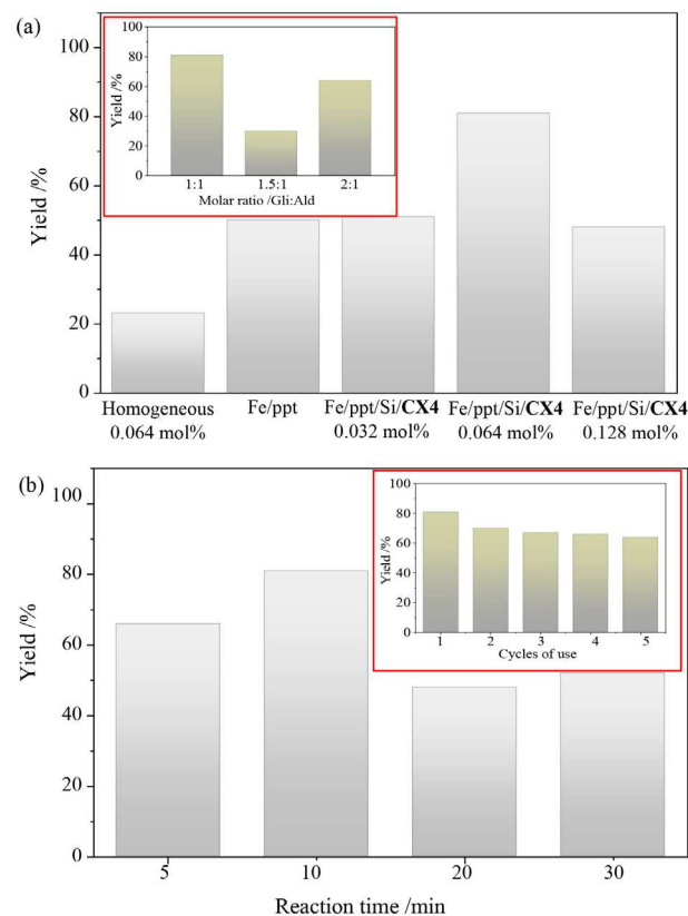
Figure 10. (a) Influence of the amount of catalyst (Fe/ppt/Si/CX4) in the reaction. The insert shows the effect of the molar ratio (glycerol/aldehyde) on yield using Fe/ppt/Si/CX4. (b) Effect of time on benzaldehyde acetalization reaction using Fe/ppt/Si/CX4. The insert shows the yield of five reaction cycles using Fe/ppt/Si/CX4. Reaction conditions: without solvent, 100 °C; MW, 10 min.
