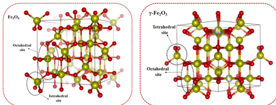
Figure 5. Three-dimensional structure of the phases \text{Fe}_3\text{O}_4 and \gamma\text{-Fe}_2\text{O}_3 . All structures were generated from the Crystallographic Information File (CIF), 72,73 taken from the Crystallography Open Database, and from Vesta (Visualization software for Electronic and Structure Analysis).
