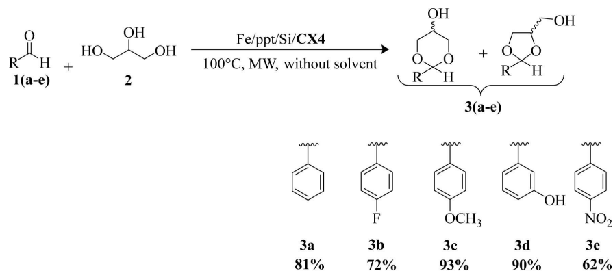
Figure 11. General scheme of the reaction with the optimized conditions and the aldehydes used to obtain the acetals.
