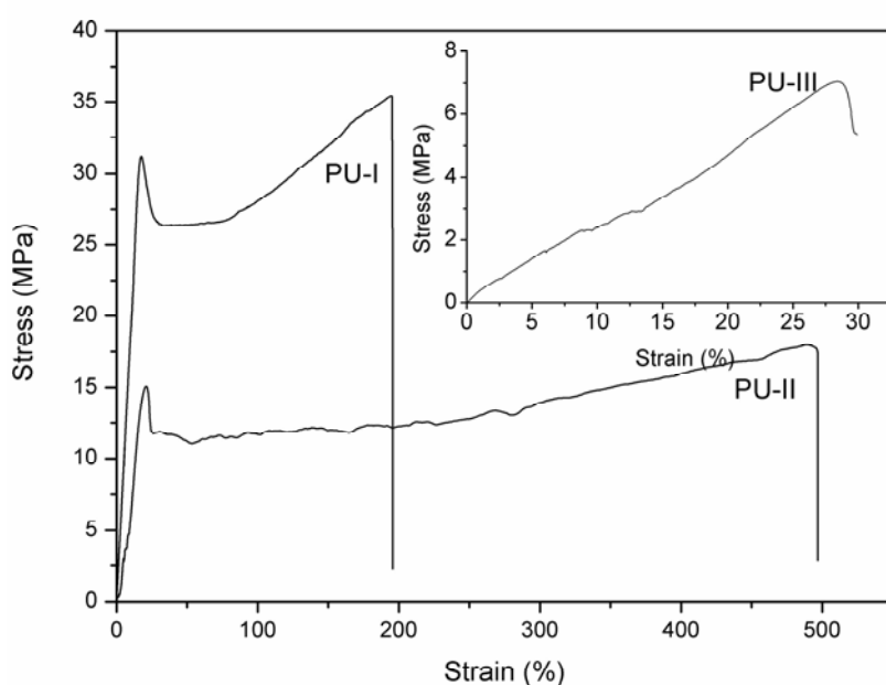
Figure VII.12 – Stress–strain curve of PU-I, PU-II and PU-III.
