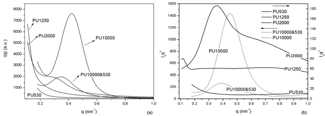
Figure II.6 – (a) SAXS curves of obtained PUs and (b) Deconvoluted Lorentz SAXS pattern of samples.
