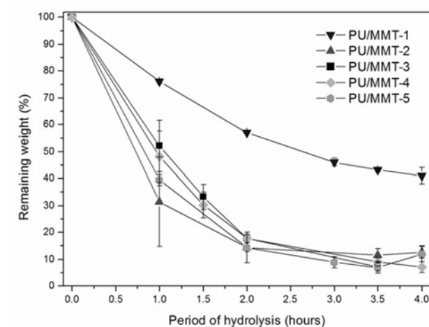
Figure IV.13 – Alkaline degradation of PU/MMT-1 to PU/MMT-5.
