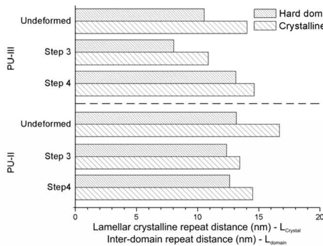
Figure VII.10 – Inter-domain repeat distance and lamellar crystalline repeat distance of PU-II and PU-III during shape memory cycle.
