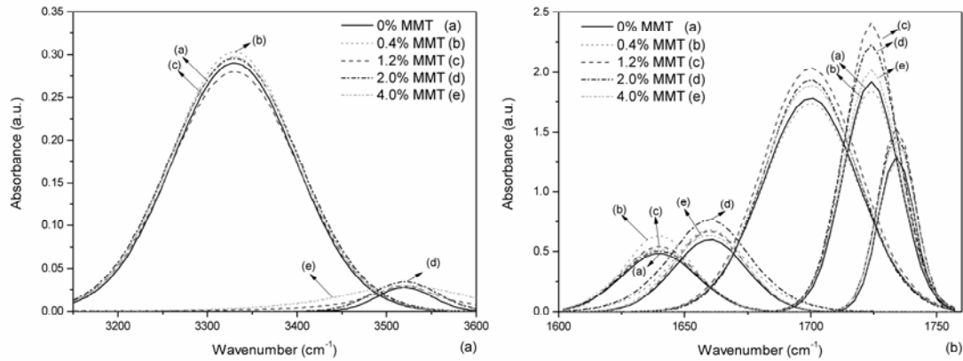
Figure IV.4 – Deconvoluted FTIR spectrum: (a) N–H stretching region, (b) carbonyl stretching region.
