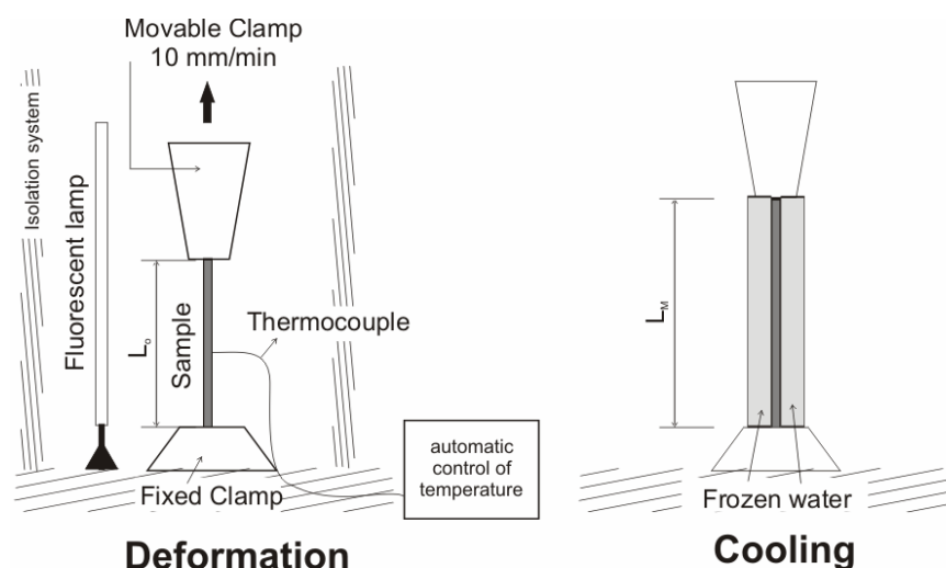
Scheme VII.1 – Shape memory test set-ups.
