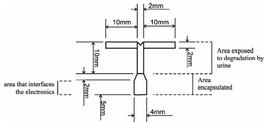
Figure IX.2 – Anchor system draft (thickness = 0.4mm)
