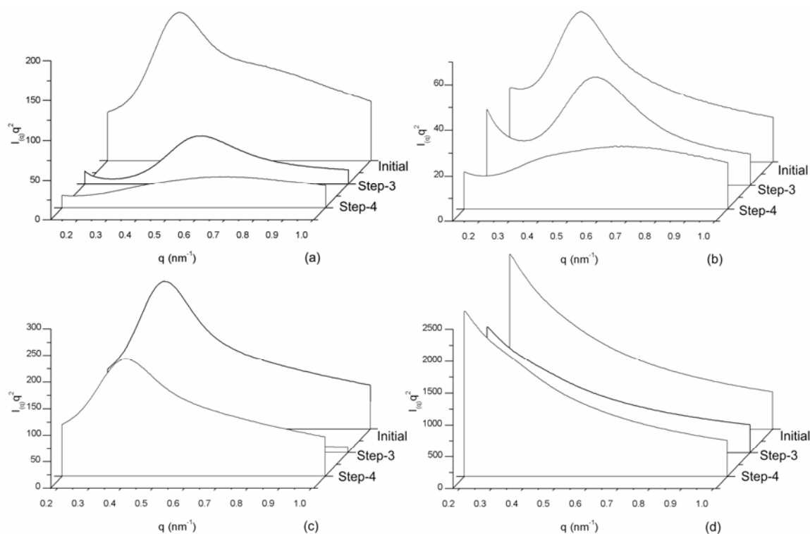
Figure VIII.4 – SAXS curves of obtained PUs: (a) PU-C, (b) MMT-1, (c) MMT-2 and (d) MMT-3
