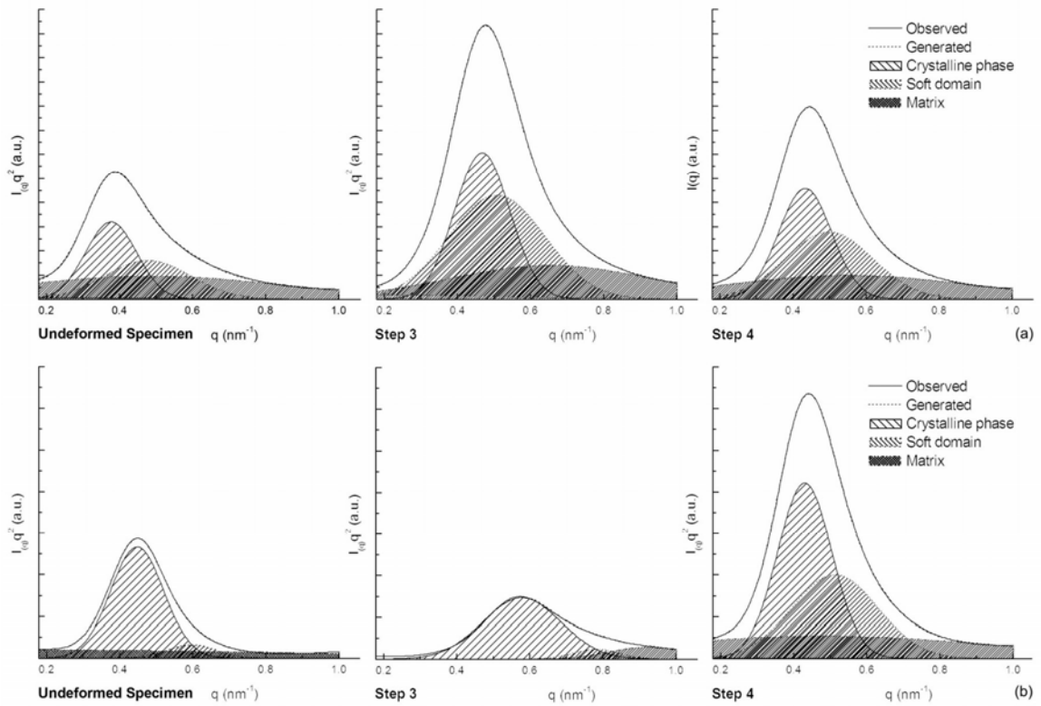
Figure VII.8 – Deconvoluted Lorentz SAXS pattern of samples: (a) PU-II, and (b) PU-III.
