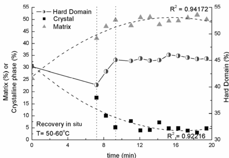
Figure V.6 – PU multi-phase evolution during in situ tests.
