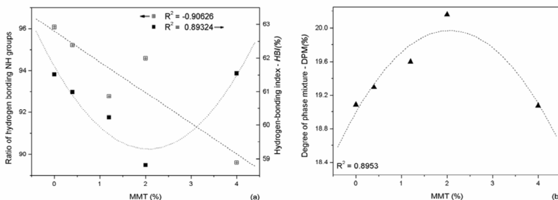
Figure IV.5 – Influence of filler content on: (a) ratio of hydrogen bonding NH groups and HBI(%) and (b) phase mixture.
