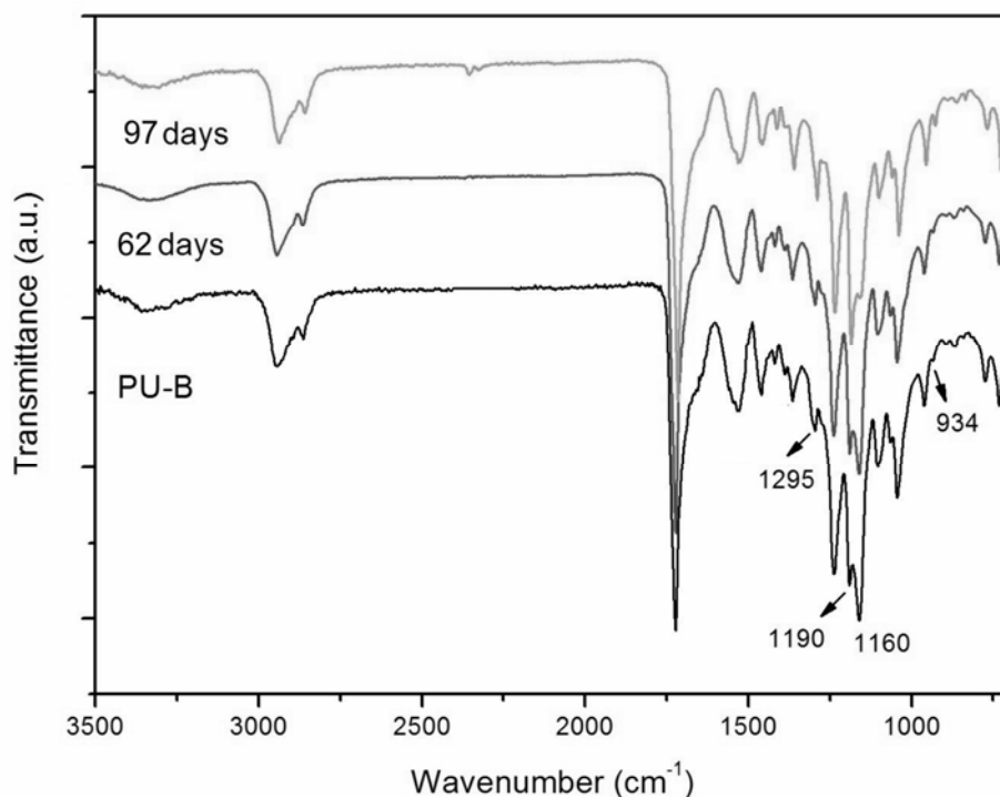
Figure III.3 – FTIR spectra of PU-B after hydrolysis performed at 37^{\circ}\text{C} in PBS for 62 and 97 days.
