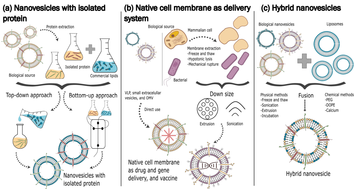
Figure 3. Design strategies for biomimetic vesicles. (a) Nanovesicles with isolated proteins are produced by top-down or bottom-up approaches by isolating a specific protein from a biological source and putting it into the lipid bilayer of a nanovesicle to confer a specific function to the delivery system. (b) Biological nanovesicles, such as small extracellular vesicles and outer membrane vesicles, can be used directly as drug or gene delivery systems; macrovesicles, such as cell and bacteria ghosts, can be extracted and downsized by extrusion or sonication for use in this application also. (c) Hybrid nanovesicles are obtained from the fusion of a biological vesicle and a synthetic liposome by physical or chemical methods in order to increase production yield.
