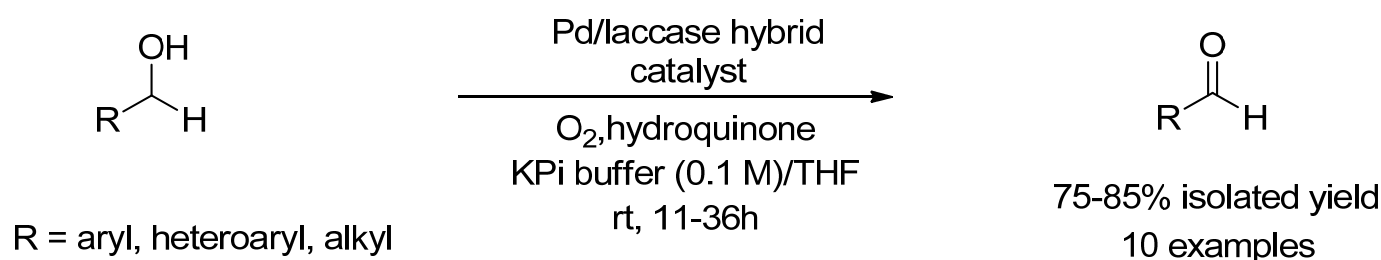
Scheme 3. Oxidation of alcohols in aqueous media catalyzed by a Pd/laccase hybrid catalyst [175].
