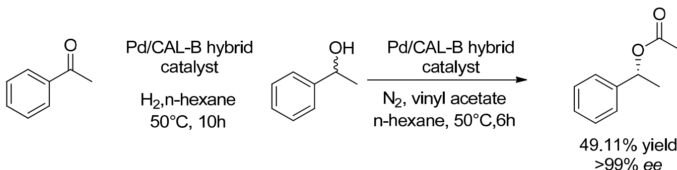
Scheme 2. One-pot reduction/kinetic resolution cascade catalyzed by a Pd/CAL-B hybrid catalyst [173].
