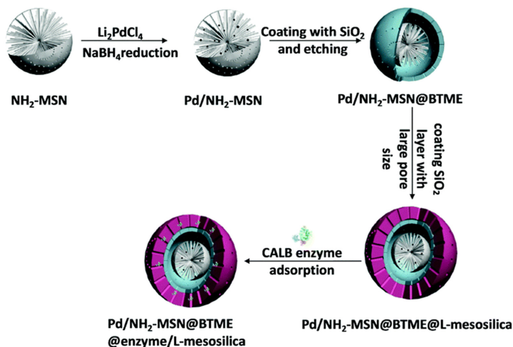
Figure 7. Preparation of a Pd/CAL-B yolk@shell-shell catalyst [175]. Reprinted from [175] with permission of Royal Society of Chemistry.
