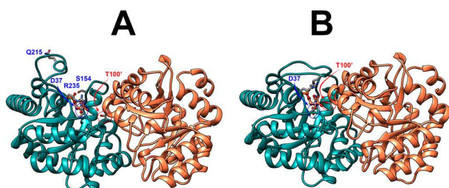
Figure 6. Representations of the open (A, PDB 3GDK) and the closed or liganded (B, PDB 3GDL) forms of yeast OMPDC where the azUMP ligand is placed at structure A at the position determined for structure B. These representations show the movements of the phosphodianion gripper loop (P202–V220) toward the pyrimidine umbrella loop (A151–T165) and R235 toward the phosphodianion, as well as the movement of the G'98–S'106 \alpha -helix from the second subunit toward the bound substrate and the pyrimidine umbrella of the main subunit. The bridging interaction between the -\text{CH}_2\text{OH} side chain of S154 and the amide side chain of Q215 at the closed enzyme is not shown.
