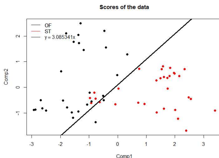
Figure 8: Frontier delimited by Fisher's discriminant function.
