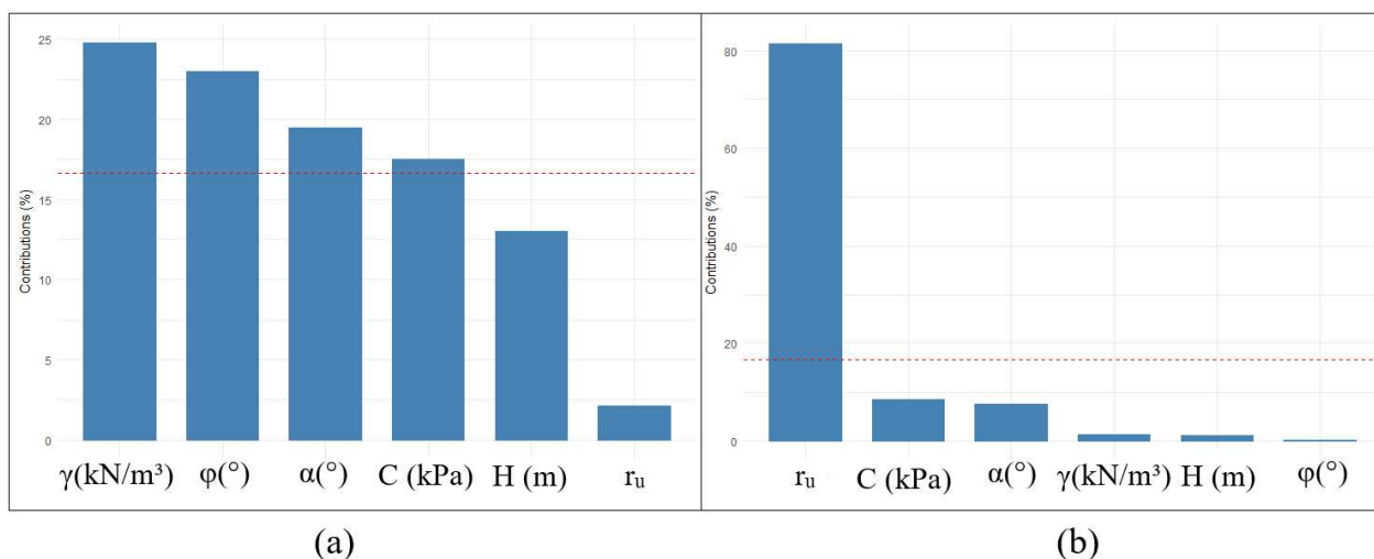
Figure 5: (a) Importance of variables in the 1 a Component; (b) Importance of variables in the 2 a Component.
