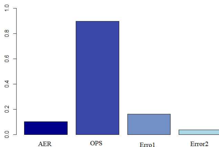
Figure 7: Cross-validation of the discriminant function.
