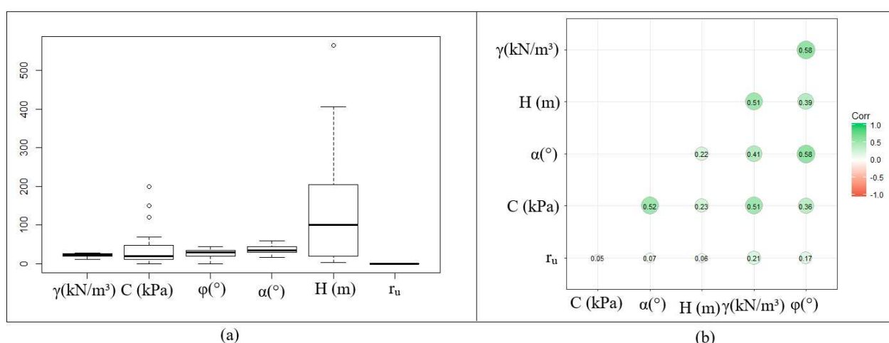
Figure 3: (a) Boxplot of the variables; (b) correlogram of the variables.
