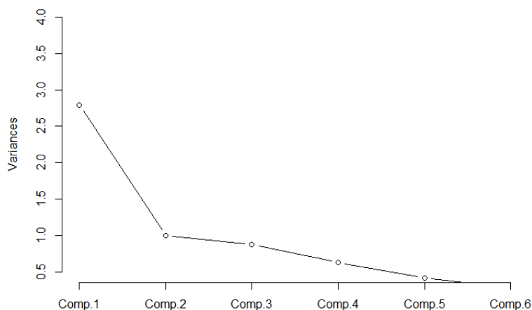
Figure 4: Screen-plot by Catell (1966).
