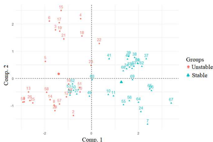
Figure 6: Scores for the first and second principal component.
