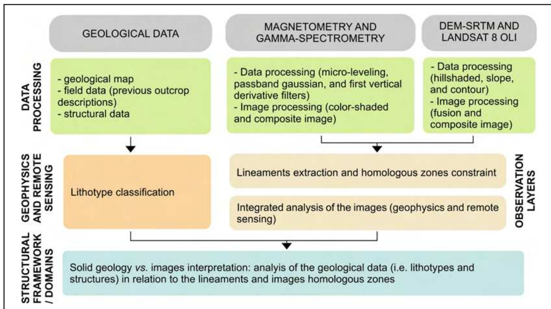
FIGURE 2. Methodological flow chart of the geological-structural modeling based on multi-source data sets.
