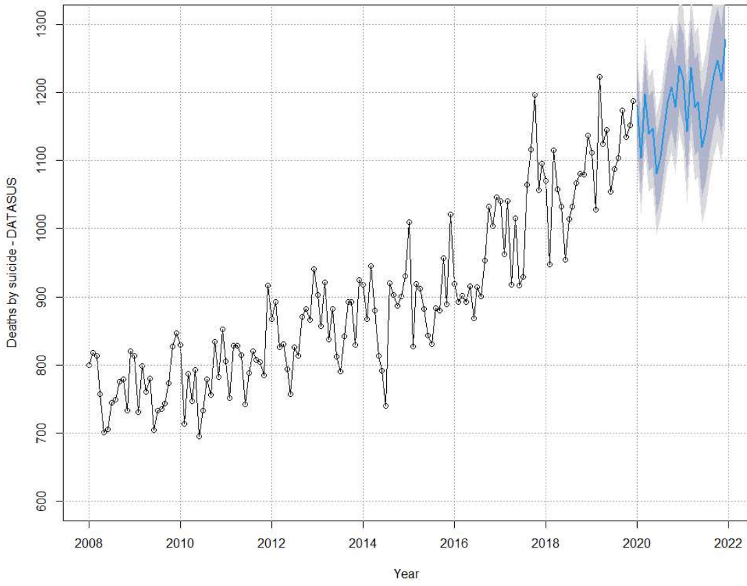
Forecast by SARIMA
