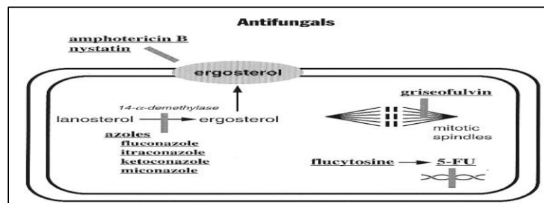
Figure 3: Mechanism of action involving the inhibition of miconazole synthesis of ergosterol (MCZ) of class Imidazole. MCZ inhibits the cytochrome P450 complex, including the enzyme 14α-demethylase required for ergosterol biosynthesis, in fungal cell membranes(39)
