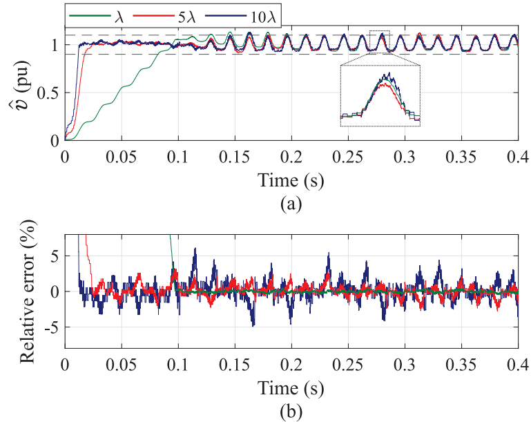
Figure 34 – Evaluation of the observer performance for different \lambda : (a) Observed voltage; (b) Relative error. Remark: the switching frequency is f_c = 1 kHz and sampling frequency is f_s = 22 kHz.
