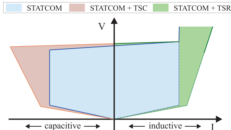
Figure 14 – VI characteristic of hybrid STATCOM with either TSC or TSR.
