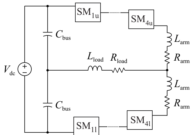
Figure 30 – Schematic of the downscaled MMC prototype.
