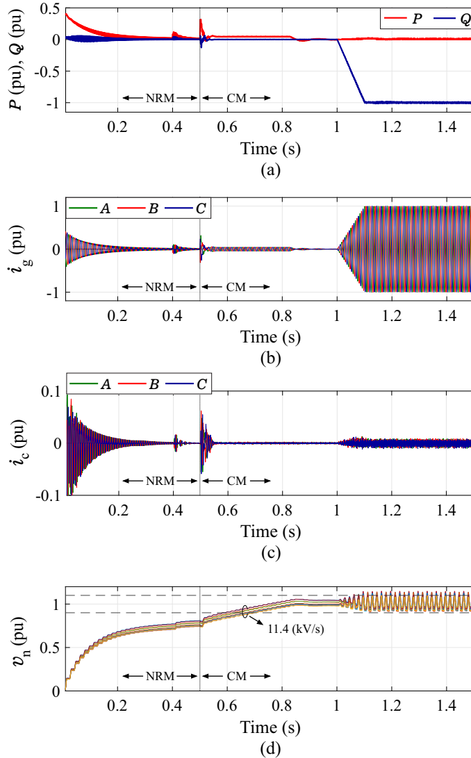
Figure 25 – Dynamic behavior of HB-MMC during energization condition: (a) Instantaneous active and reactive powers; (b) Grid currents; (c) Circulating currents; (d) SM capacitor voltages.
