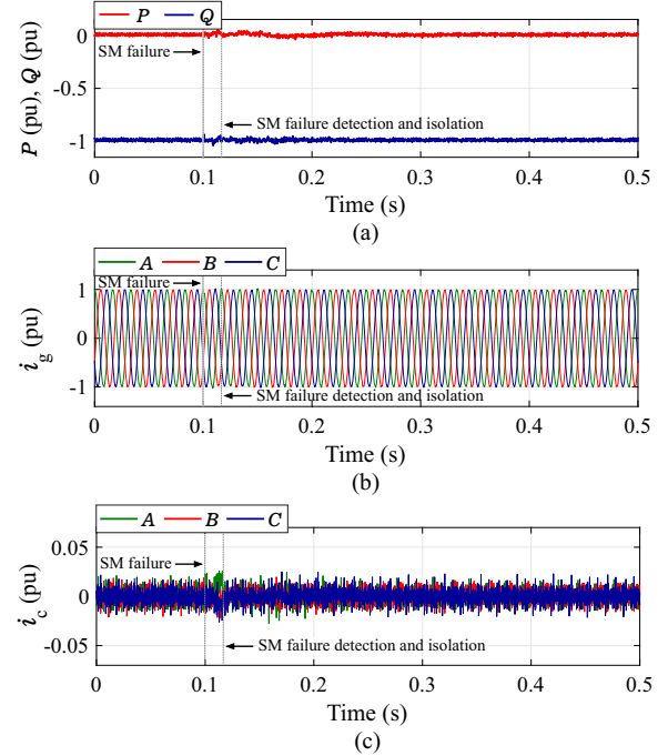
Figure 55 – Dynamic behavior of HB-MMC considering AR method: (a) Instantaneous active and reactive powers; (b) Grid currents; (c) Circulating currents.
