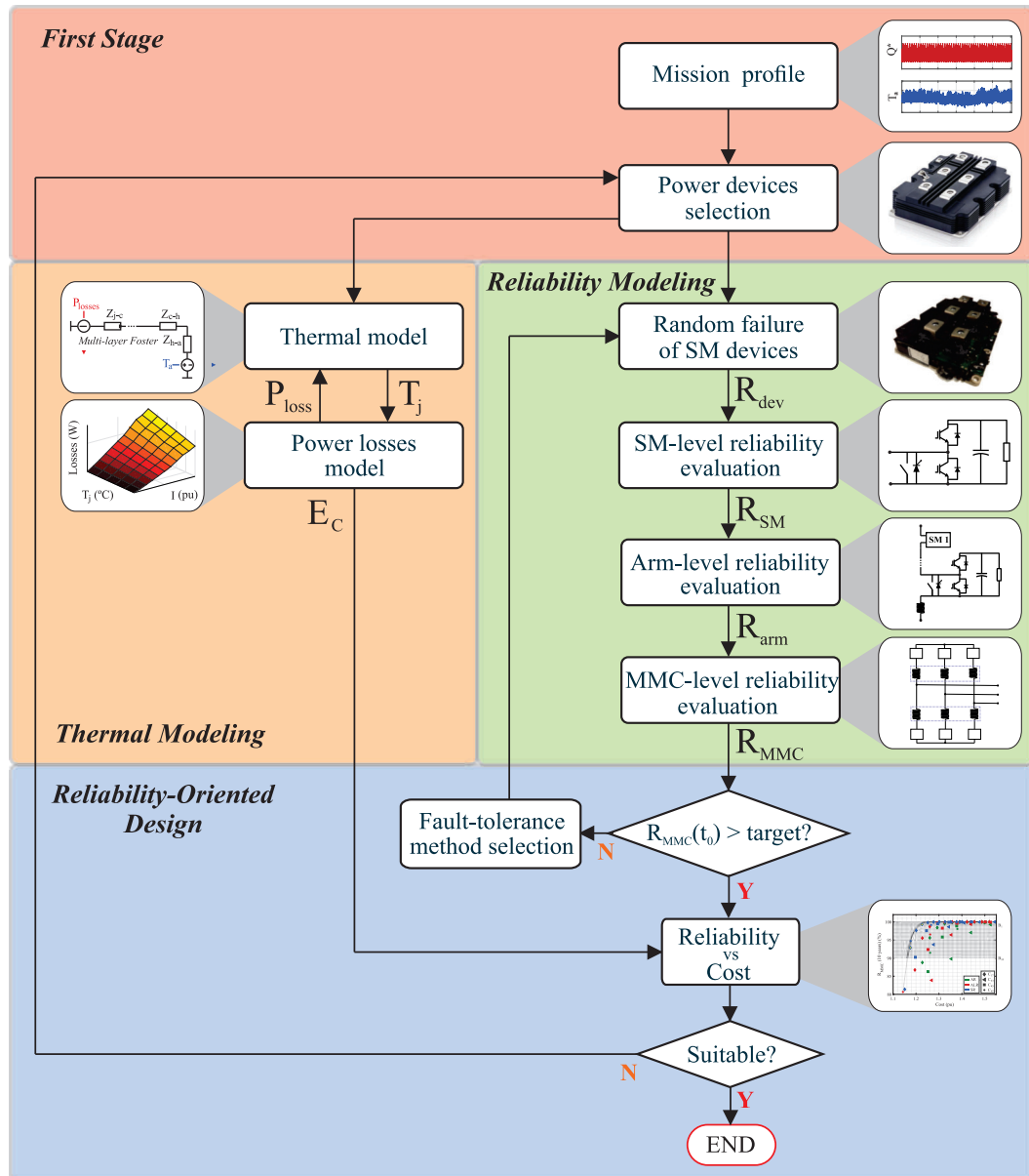
Figure 66 – Flowchart of the reliability-oriented design.
