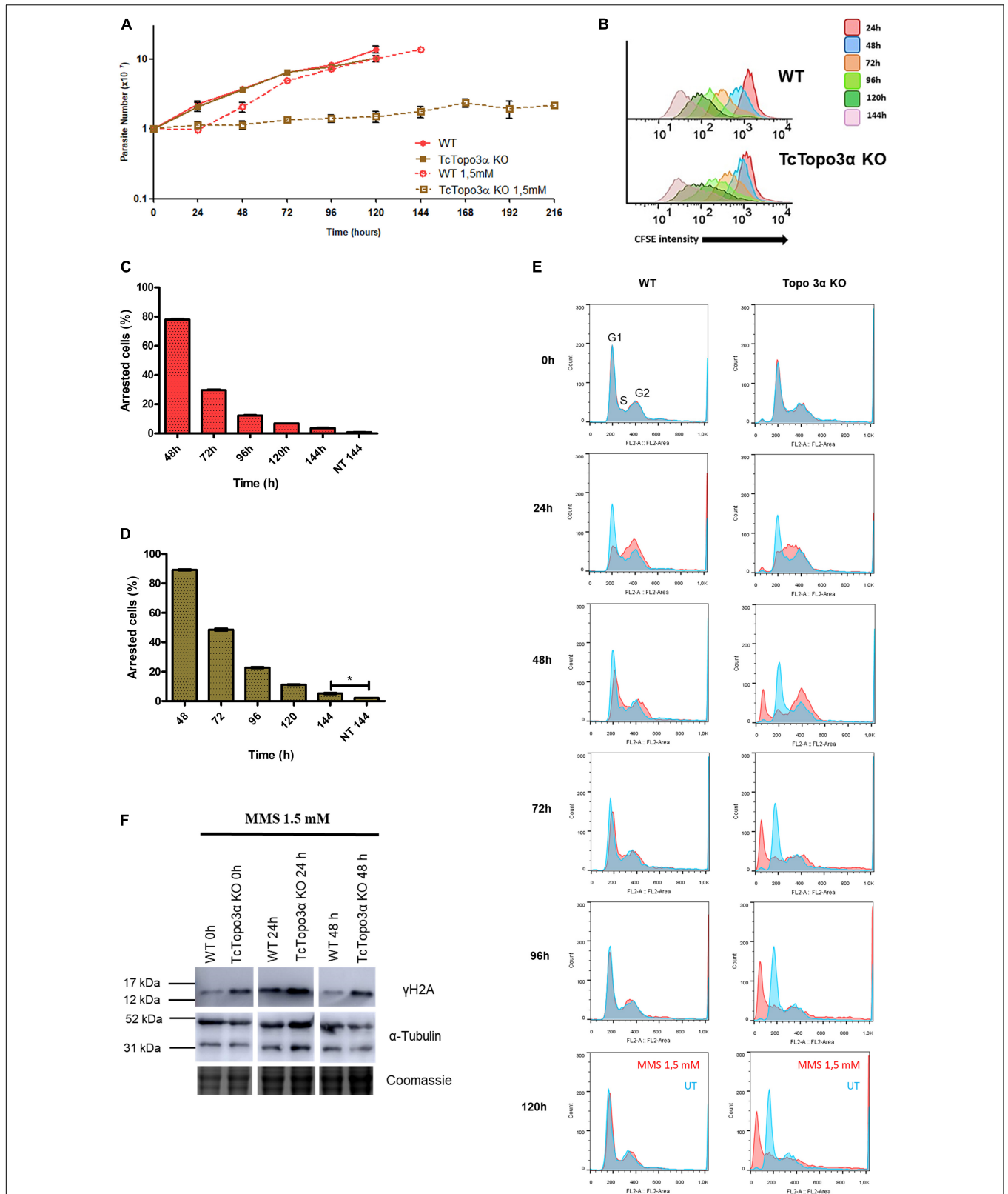
FIGURE 6 | The role of topoisomerase 3α in the response to methyl methanesulfonate (MMS) treatment. (A) Growth curve after the treatment with 1.5 mM MMS for 1 h in PBS buffer. After the treatment, the cells were cultivated in fresh medium. The cells were counted every day using a cytometry chamber and vital dye (Continued)
