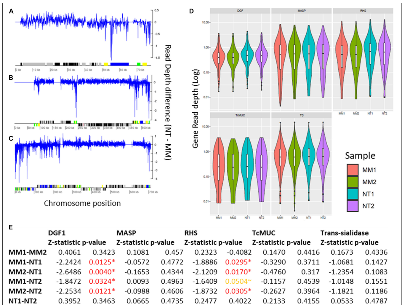
FIGURE 7 | Impact of MMS treatment in segmental and gene duplication/loss in TcTopo3 \alpha KO cells. Segmental duplications in Chromosomes 1 (A) , 12 (B) , and 22 (C) . In this image, the blue line corresponds to the difference between the read depth of NT (1–2) and MM (1–2) across the whole chromosome sequence, where values above and below zero correspond, respectively, to increase copies in MM (1–2) and NT (1–2). Below, protein-coding genes are depicted as rectangles drawn in proportion to their length, and their coding strand is indicated by their position above (top strand) or below (bottom strand) the central line. Colored boxes represent: DGF-1 (blue); GP63 (Pink); MASP (brown); RHS (green); and Trans-sialidase (yellow); hypothetical genes (black); or other genes (gray). Gaps are represented by gene-less regions with no read coverage. (D) Violin plot representing the gene copy number of DGF-1, MASP, RHS, TcMUC, and Trans-Sialidase genes. The Y-axis represents the distribution of gene coverages, in log scale. MM1 (red), MM2 (green), NT1 (blue), and NT2 (purple). (E) Z-statistic and p-values of Dunn's test between the comparisons of DGF-1, MASP, RHS, TcMUC, and trans-sialidase gene coverages. P-values < 0.05 are highlighted in red, and p-values ~0.05 are highlighted in orange. There was a significant reduction in the DGF-1 and RHS copy numbers in MMS-treated TcTopo3 \alpha KO isolates.
