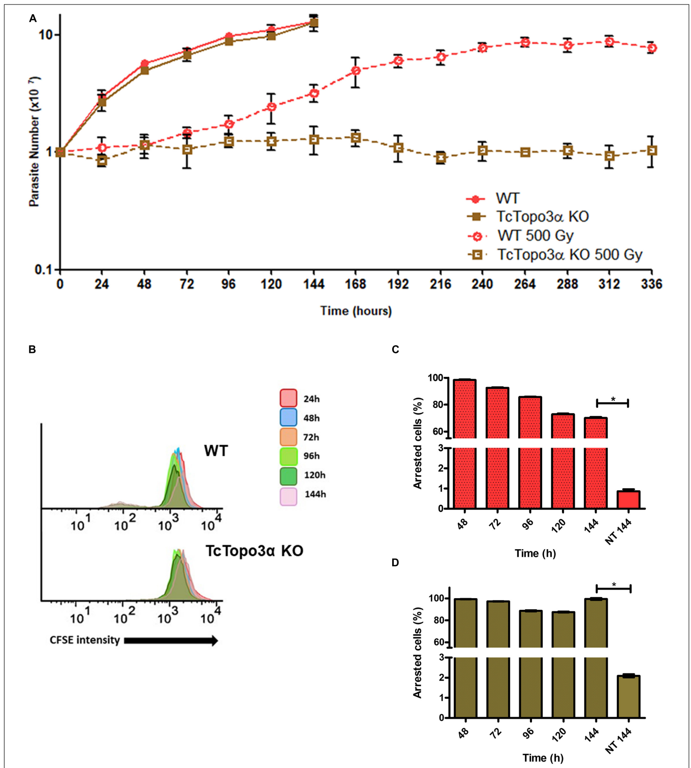
FIGURE 3 | Growth curve and dormancy after gamma radiation. (A) Evaluation of the growth profile of WT and TcTopo3 \alpha KO T. cruzi epimastigotes parasites after exposure to 500 Gy of gamma radiation. The parasites were cultured in LIT medium at initial concentration of 1 \times 10^7 cells \text{ml}^{-1} and counted in a cytometry chamber every 24 h. The experiment was performed in triplicate. (B) Flow cytometry histograms of CFSE fluorescence intensity decay over time from epimastigotes exposed to 500 Gy. Cells that have similar CFSE fluorescence intensity compared with the level of half median at time point of 24 h were considered as arrested. (C,D) The graph shows the percentage of WT (C) or TcTopo3 \alpha KO (D) arrested parasites determined by flow cytometry showing half of CFSE median intensity observed at 24 h of growth. The percentage of dormant parasites at 144 h – from a culture without exposure to HU (NT 144 h) is shown for the sake of comparison. Representative results of three distinct experiments in three technical triplicates. Asterisks indicate statistically significant differences among groups ( p -value < 0.05).
