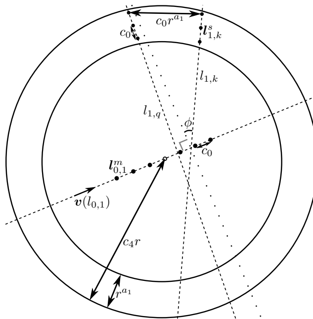
Figure 2: Construction of the first layer. Dashed lines represent the “given” l_0 in \mathbf{L}_0 , and two lines l_{1,k} and l_{1,q} from threads k and q \neq k in \mathbf{L}_1 , respectively. The image is a projection onto a flat surface which is parallel to l_{1,k} and l_0 . We demand that \phi = \arcsin\langle v(l_0), v(l_{1,k}) \rangle \in [\alpha, \beta] . Filled dots on the picture are “beads” lying on l_0 , l_{1,k} and l_{1,q} .
