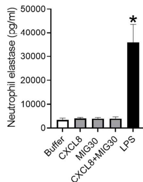
Figure 5. The MIG30 peptide does not affect the responsiveness or activation status of leukocytes towards stimuli. (A) Intracellular calcium signal ([Ca 2+ ] i in nM) in purified human neutrophils loaded with Fura-2/AM and stimulated with CXCL8 (10 ng/mL) and/or MIG30 (20 µg/mL). Results
