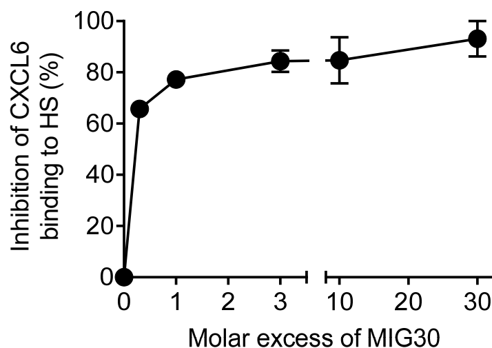
Figure 1. MIG30 inhibits the binding of CXCL6 to heparan sulfate GAGs. Competition between CXCL6 and MIG30 peptide for binding to immobilized heparan sulfate was evaluated on 96-well plates. CXCL6 (300, 100, 30, 10 and 3 nM) was added to heparan sulfate plates in the presence/absence of MIG30 (CXCL9(74-103); 100 nM). Bound CXCL6 was detected with biotinylated anti-mouse CXCL6 antibody. The data shown are the mean \pm SEM of the percent of inhibition compared to CXCL6 binding alone.
