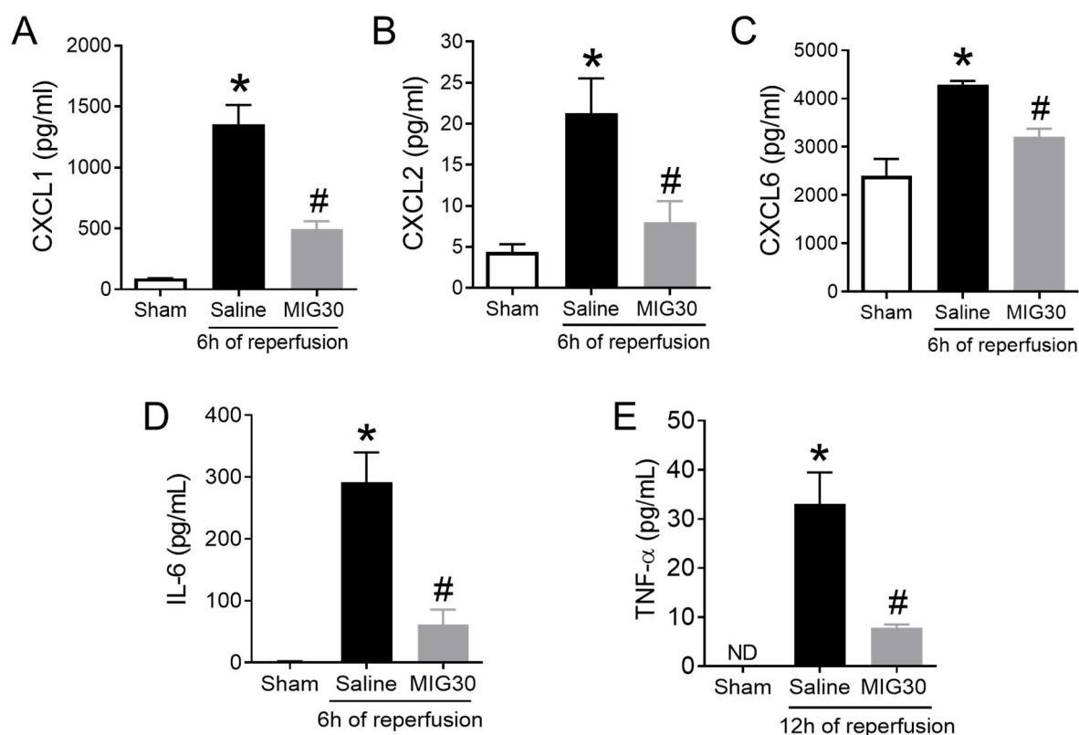
Figure 4. The levels of CXC chemokines and proinflammatory cytokines are reduced in MIG30-treated mice. Quantification of (A) CXCL1, (B) CXCL2, (C) CXCL6, (D) IL-6 and (E) TNF- \alpha in the sera of mice subjected to liver IRI. Sham operated mice were used as control. IRI mice were either treated with saline vehicle or with MIG30 peptide (100 \mu g 15 min before the reperfusion and again 6 h later, i.v.). CXCL1, CXCL2, CXCL6 and IL-6 were measured at 6 h of reperfusion. TNF- \alpha was measured 12 h post reperfusion. ND = Not detected. The data shown are the mean \pm SEM; n is at least 4 mice per group. * p < 0.05 vs. sham group; # p < 0.05 vs. saline-treated mice.
