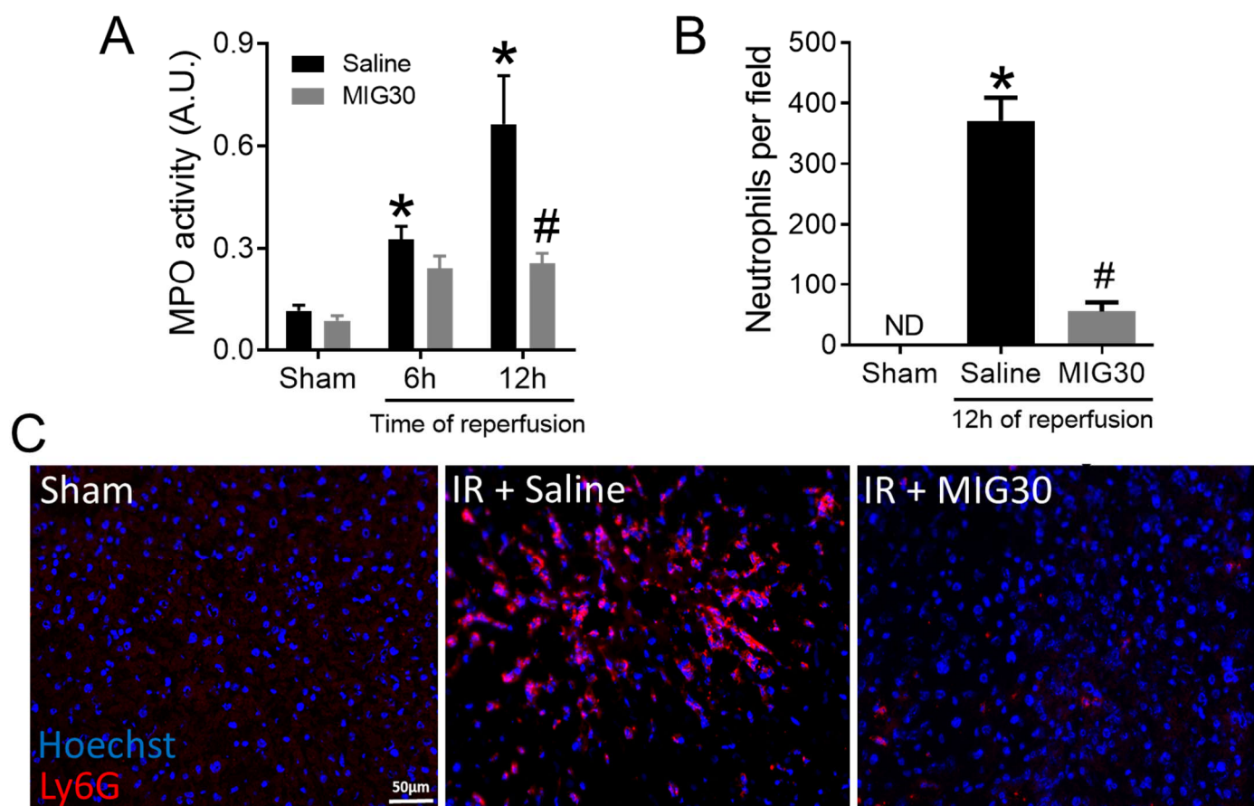
Figure 3. MIG30 treatment impairs neutrophil recruitment during liver IRI. (A) Liver MPO activity in mice subjected to liver ischemia-reperfusion injury (IRI). Sham operated mice were used as control. IRI mice were treated i.v. with saline vehicle or with MIG30 (100 μg 15 min before the reperfusion and again 6 h later). (B,C) Immunostaining of liver cryosections with anti-Ly6G to show recruited neutrophils. Neutrophils (Ly6G + ) are shown in red and Hoechst-stained nuclei in blue. (B) The data shown are the averaged number of neutrophils per field of view. (C) Representative photomicrographs of Ly6G + neutrophils in sham, mice subjected to IR and treated with saline or IR-injured mice treated with MIG30. ND = Not detected. The data shown are the mean ± SEM; n is at least 4 mice per group. * p < 0.05 vs. sham group; # p < 0.05 vs. saline-treated mice. Scale bar = 50 μm.
