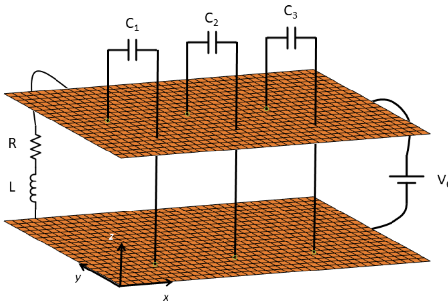
Figure 4.2: Illustration of the power bus bar model.
