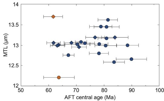
Fig. 7. AFT age – mean track length (MTL) or “boomerang plot”. As track lengths are mostly similar, there is no clear trend showing. Disregarded samples BR-12 and BR-20 are marked in orange.
