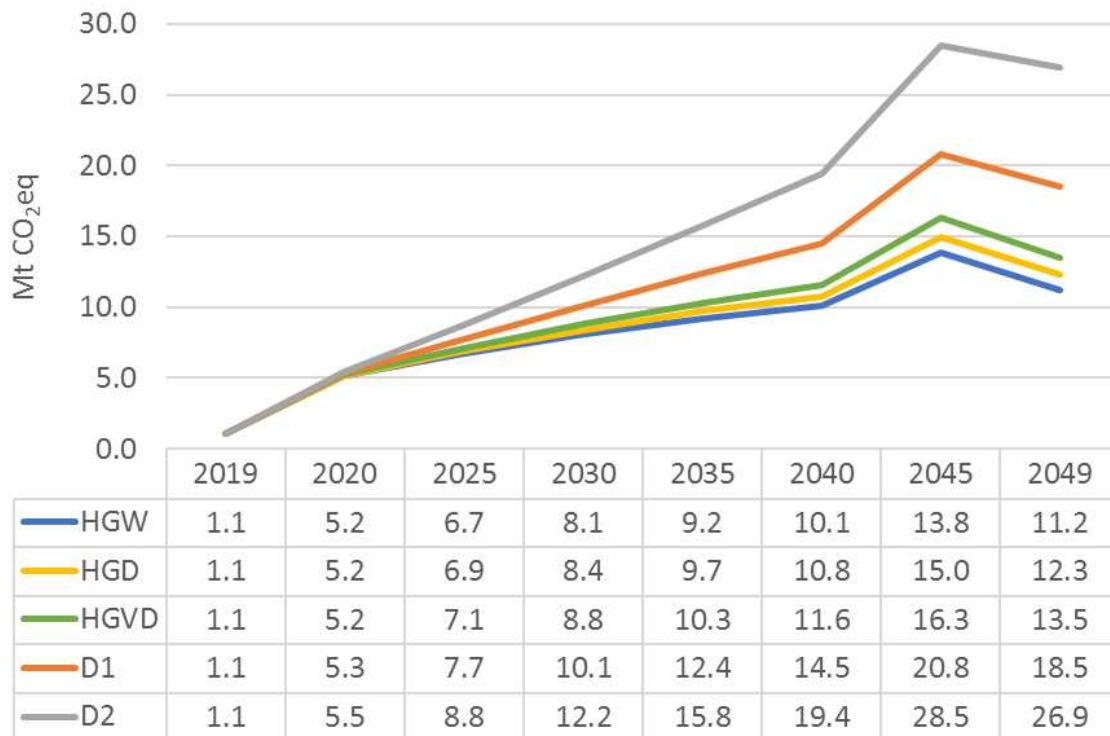
Figure 5: GHG emissions - results for all scenarios.
