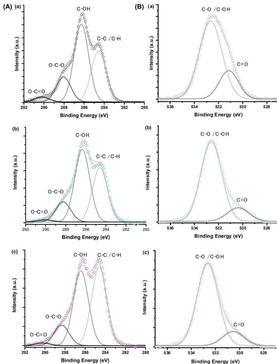
Fig. 4 XPS spectra of (A) C 1s and (B) O 1s regions obtained for (a) CMC ligand, (b) MION@CMC, and (c) Co 10 -MION@CMC.
