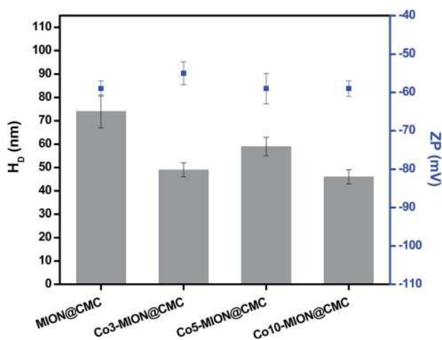
Fig. 6 DLS and ZP results obtained from MION@CMC and Co x -MION@CMC at pH = 6.5 \pm 0.5 and conductivity = 420 \pm 10 \mu\text{S} ( n \geq 10 ; mean \pm standard deviation, SD).
