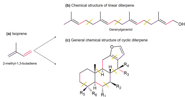
Fig. 2. Chemical structure of (a) isoprene and isolated diterpenes from Pterodon sp. (b) linear structure of Geranylgeraniol and (c) cyclic structure of vouacapan compounds. Dashed lines indicate where the four isoprene units are joined.
