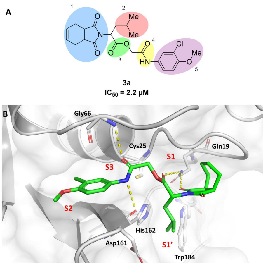
FIGURE 1 | (A) Compound 3a was used as the initial hit for the design of imide derivatives as novel cruzain inhibitors with anti- T. cruzi activity. (B) Molecular docking-predicted binding conformation of compound 3a within the active site of cruzain. Cruzain (PDB 3KKU, 1.28 Å) is depicted in cartoon and surface representations. Binding site residues (carbon in gray) and compound 3a (carbon in green) are shown as sticks. Hydrogen bonds are shown as dashed lines. Cruzain subsites are labeled as S1, S1', S2, and S3.
