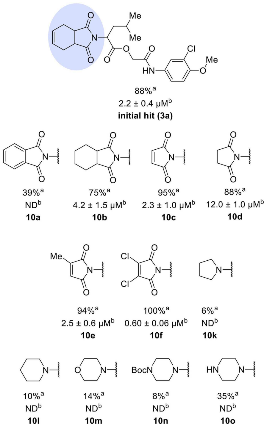
FIGURE 2 | Activity of the series of analogs featuring modifications in the imide nucleus against cruzain. a Percent inhibition against cruzain at 100 μM corresponding to the mean of three measurements. b IC 50 values against cruzain, which were independently determined by obtaining rate measurements in triplicate for at least six inhibitor concentrations. The IC 50 values represent the mean ± SD of three individual experiments. ND, IC 50 not determined.
