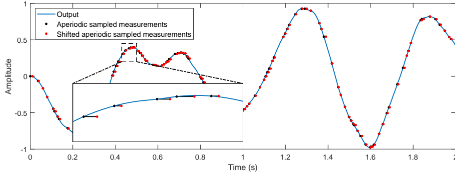
Figure 4.8: Effect of approximating the random time instants of the aperiodic sampling. Black dots are the true measurements and the red dots are the measurements shifted to the next multiple of T = 0.001 .
