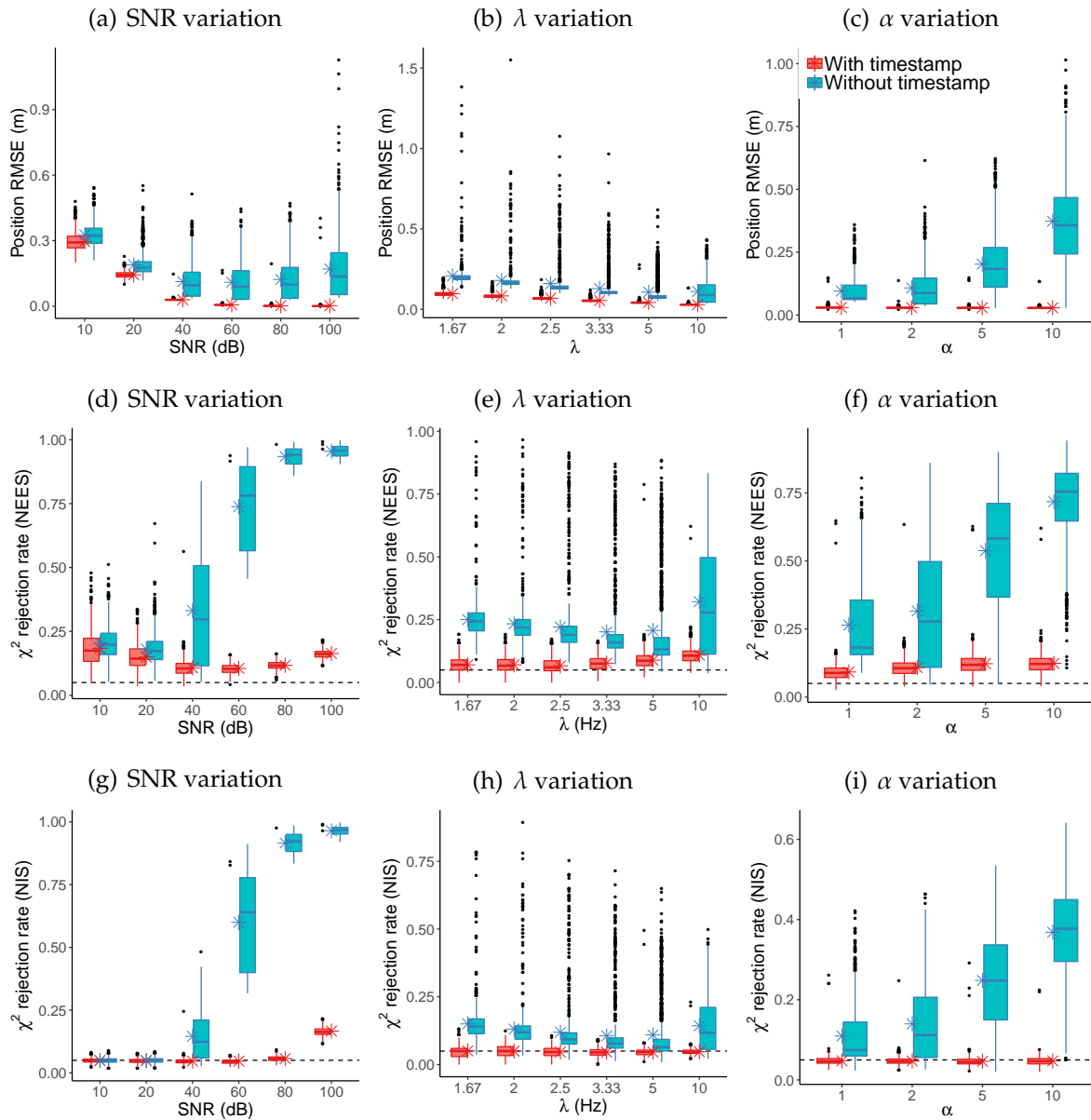
Figure 5.16: Box and whiskers plots for the nonlinear system estimation results, as a function of SNR (a,d,g), \lambda (b,e,h) and \alpha (c,f,i), considering (red) and not considering (blue) timestamps. Mean values are presented in asterisks. Horizontal gray dashed lines for consistency results represents the 5% significance level limits.
