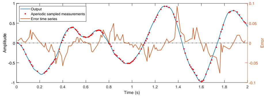
Figure 5.1: Added error time series (orange) as an effect of shifting time instants of the measurements (red) and output (blue). A gray dotted horizontal line is placed at the origin, for reference. Right scale (in orange) refers to the error data, whereas left scale (in black) refers to the output signal amplitude.
