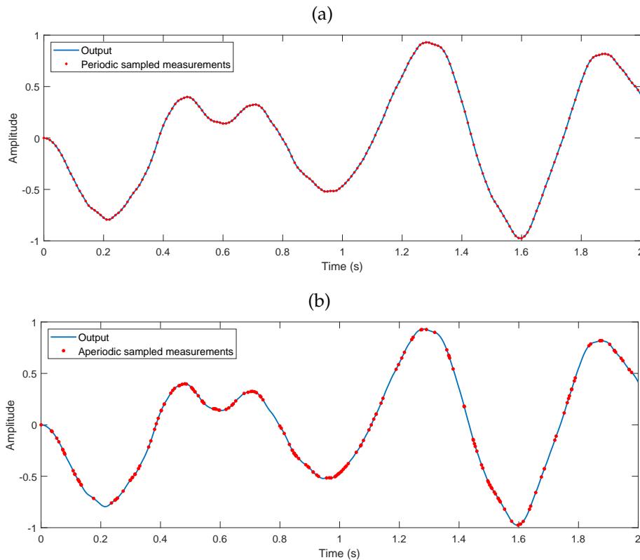
Figure 4.7: Periodic (a) and aperiodic (b) sampling of the output variable of G(s) . Aperiodic sampling instants sequence generated by a Poisson process with intensity \lambda = 100 Hz.
