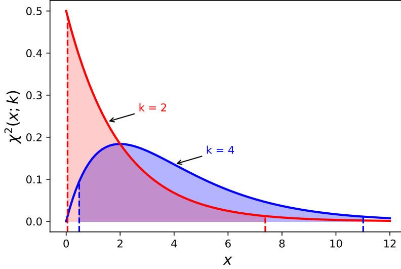
Figure 4.9: \chi^2 PDFs for 2 (red) and 4 (blue) degrees of freedom. The vertical dashed lines represent the acceptance interval limits, for \alpha = 5\% , and the shaded area is the corresponding acceptance regions.
