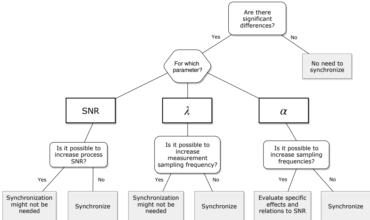
Figure 6.2: Summarized example of possible decisions derived from applying the proposed framework.
