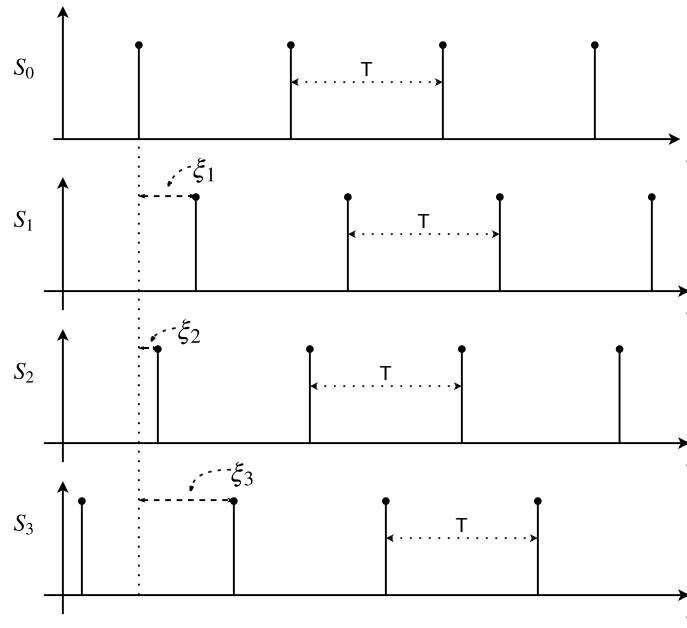
Figure 4.4: Sampling instants of four sensors ( S_i ) and their phases. The phase \xi_0 is considered to be zero. The time interval for all of them is constant and equal to T .
