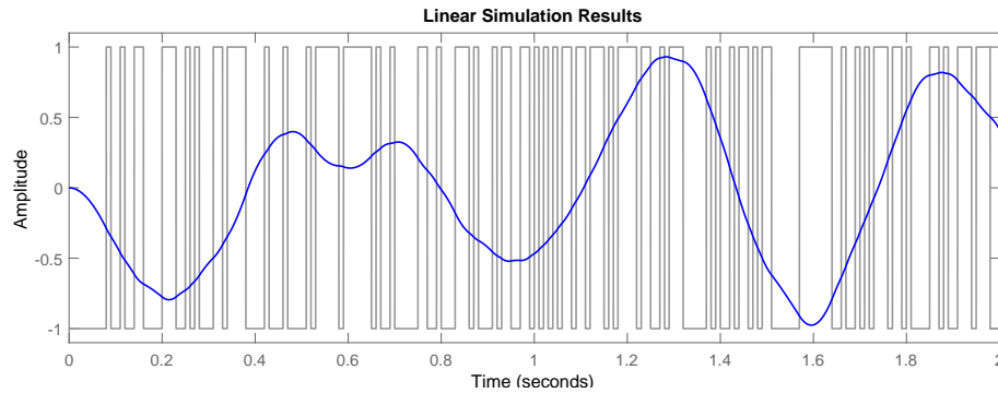
Figure 4.6: Linear simulation results for G(s) in blue, considering the PRBS input in grey.
