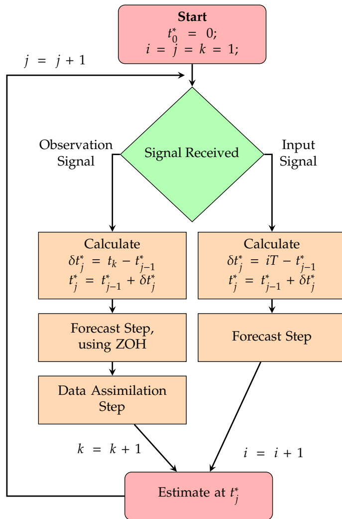
Figure 4.5: Illustrative schematic of the online estimator, with timestamp. indices i, j e k represent the input, estimation and observation signal counters, respectively.
