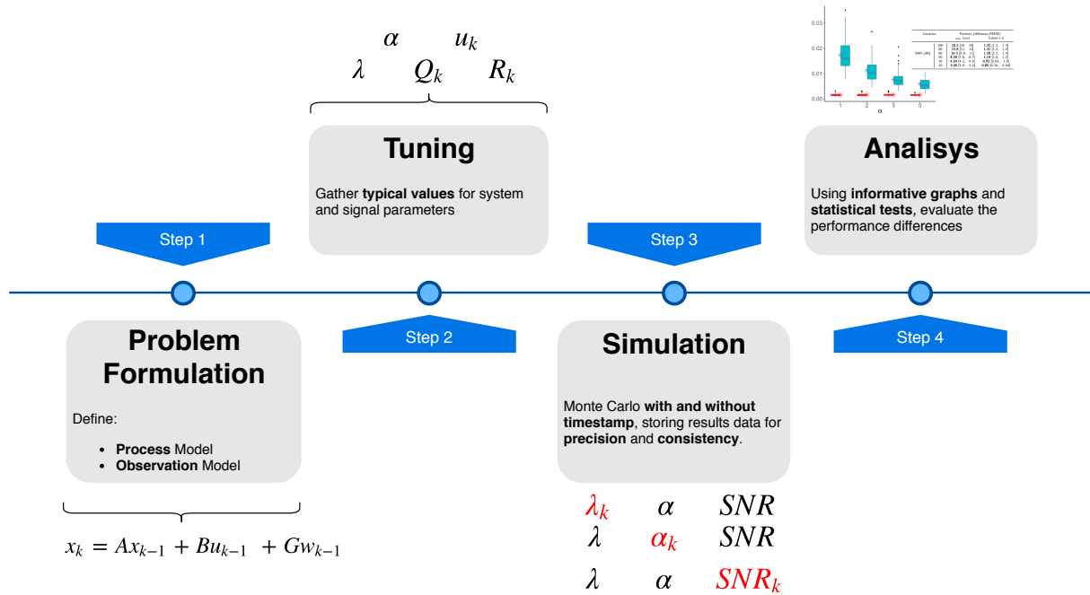
Figure 6.1: Proposed framework steps to assist decision making process for investments in sensor networks and synchronization.
