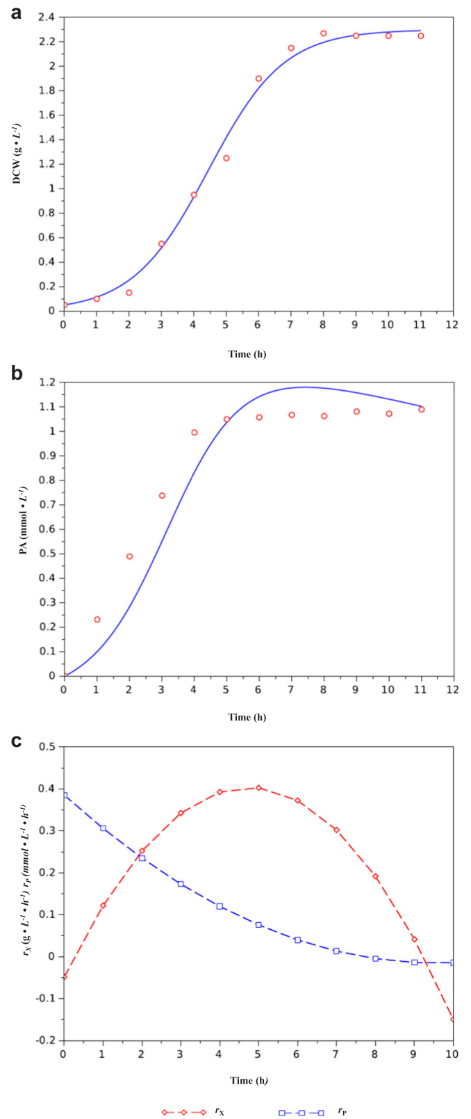
Fig. 5. Predicted data versus observed data from p3 cultivated in a stirred tank reactor (STR) under microaerobic system for the DWC growth (a), PA production (b) and fermentative parameters ( r_X ) and ( r_P ) (c).
