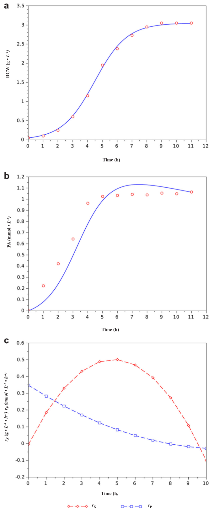
Fig. 4. Predicted data versus observed data from p3 cultivated in a stirred tank reactor (STR) under aerobic system for the DWC growth (a), PA production (b) and fermentative parameters ( r_X ) and ( r_P ) (c).
