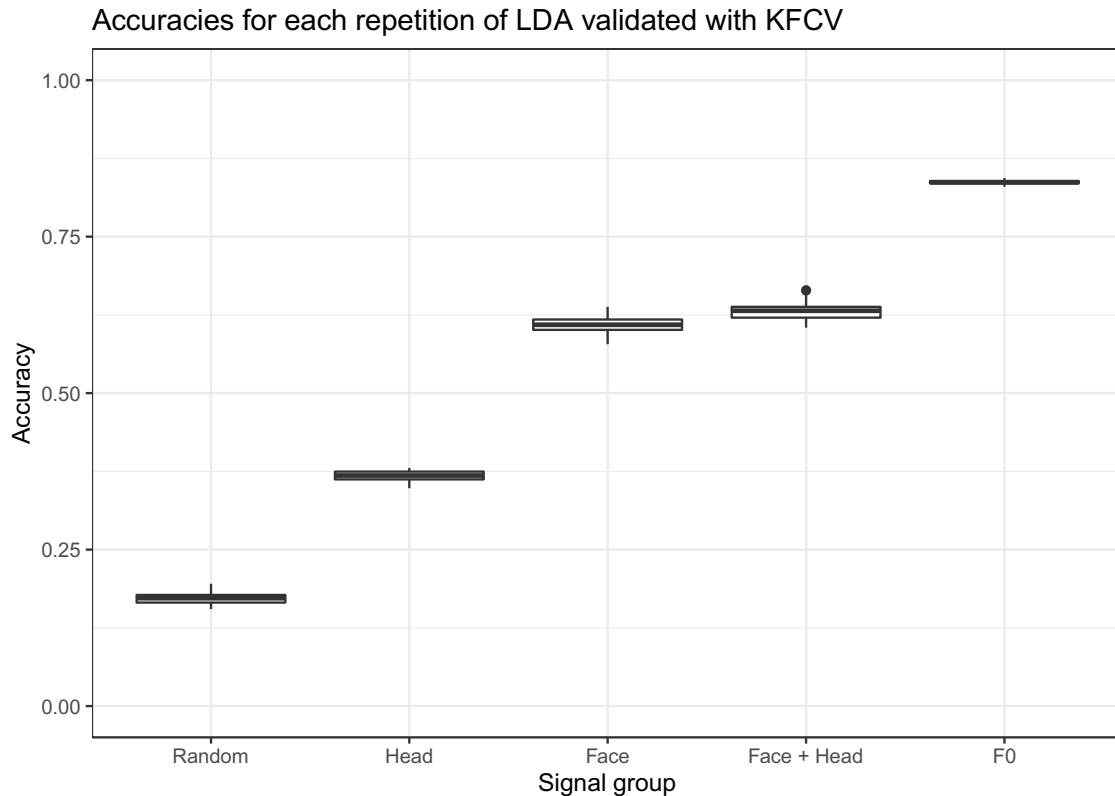
Figure 5: Box plot of the accuracies obtained in LDA classification for each signal group. Since the KFCV was repeated 60 times, each signal group is represented by 60 accuracy values, each of whom is a mean of the K = 5 accuracies obtained by each fold.
