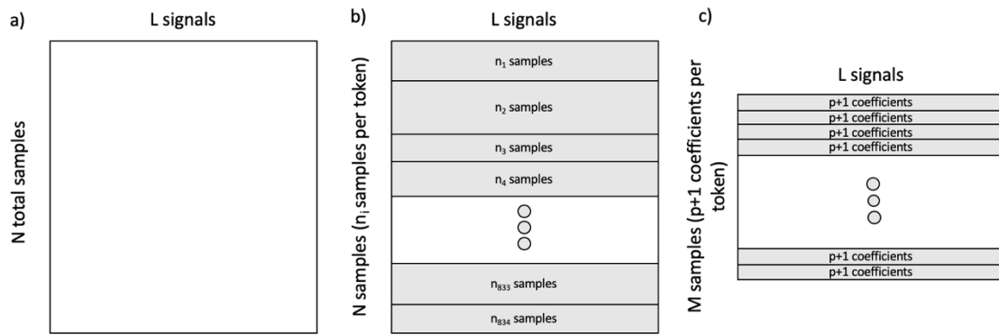
Figure 3: Generic composition of the signals of each signal group described in Table 1. a) The whole data, with N samples of L signals. b) Each token has a different number of samples ( n_i ) for each signal. c) The data after the fitting of polynomial curves. The total number of samples is now M = 834 \times (p + 1) and the length of each token's signal is (p+1) .
