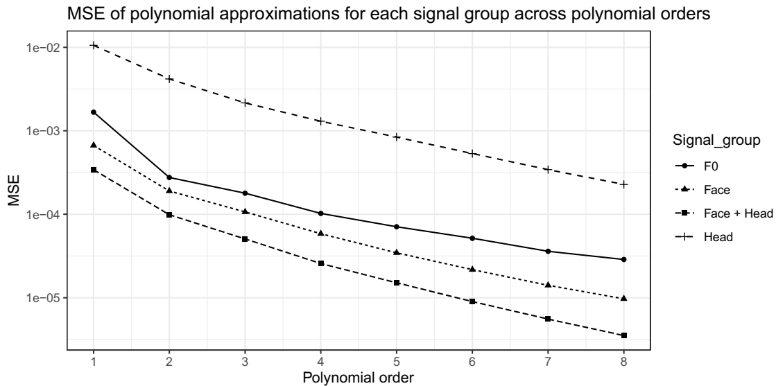
Figure 4: MSE for the polynomial approximations of each signal group. Polynomial orders varied from 1 to 8. Each value is the mean MSE over all signals of each signal group (view Table 1). The y axis is in logarithmic scale for visual clarity.
