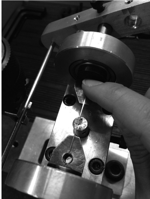
Fig. 1: Universal testing machine with the wire-bracket system positioned for torsion test.
