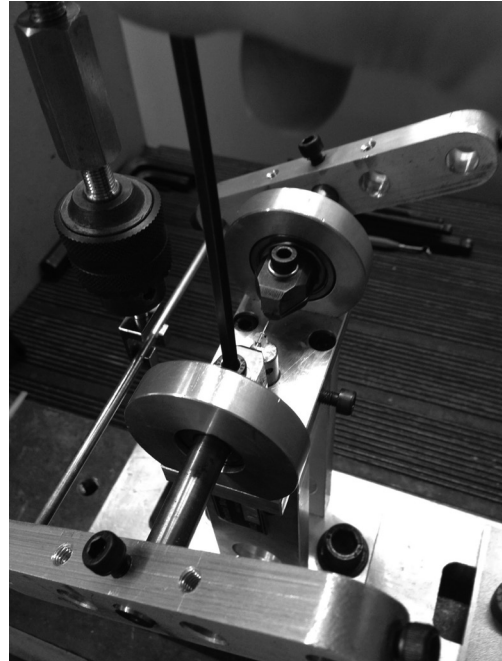
Fig. 3: The system attached by screws to avoid slipping of the set that could impair the results.
