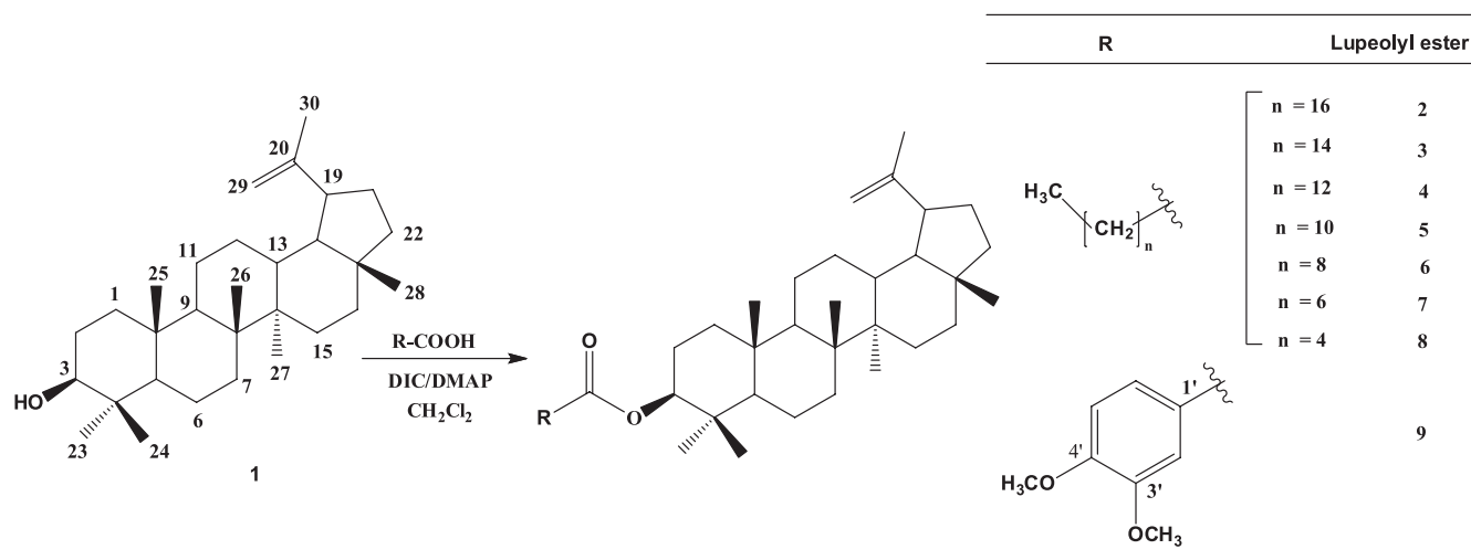
FIGURE 1 - Scheme of lupeol ( 1 ) esterification using DIC/DMAP reagents, to obtain lupeol esters 2 to 9 .
