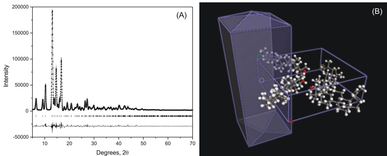
FIGURE 2 - Powder X-ray diffraction (XRD) data: (A) lupeol diffractogram; (B) lupeol chemical structure, found in solid with a needle shape.
