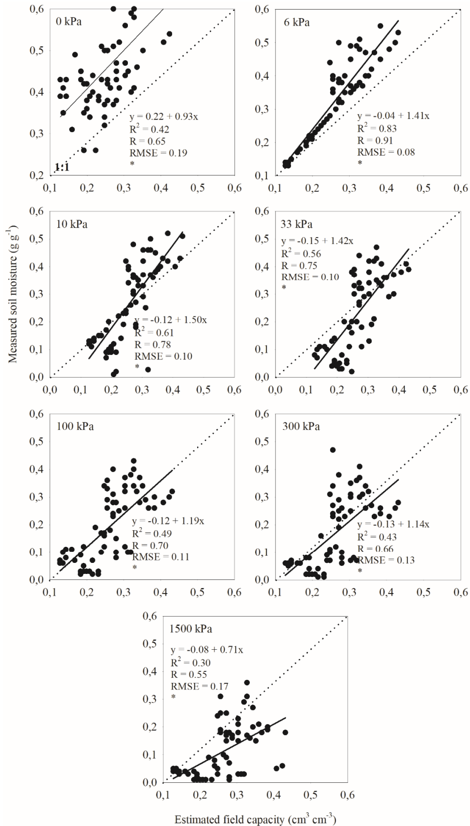
Figure 5. Linear regression between field capacity (FC) estimated using PF3 and soil moisture measured at different tensions (KPa): 0, 6, 10, 33, 100, 300, and 1500. The dotted line represents the 1:1 regression line. *p<0.001 (F test).
