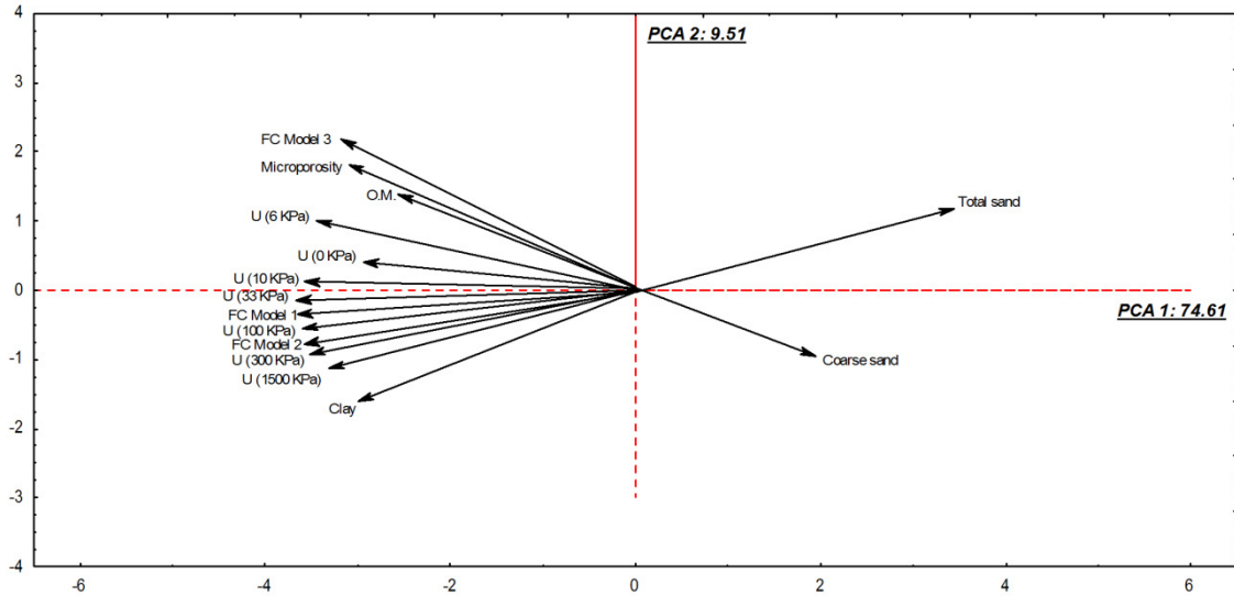
Figure 2. Principal component analysis (PCA 1 and PCA 2) of the soil attributes and FC estimated by PTFs 1, 2, and 3 (the order is represented by the arrows).
