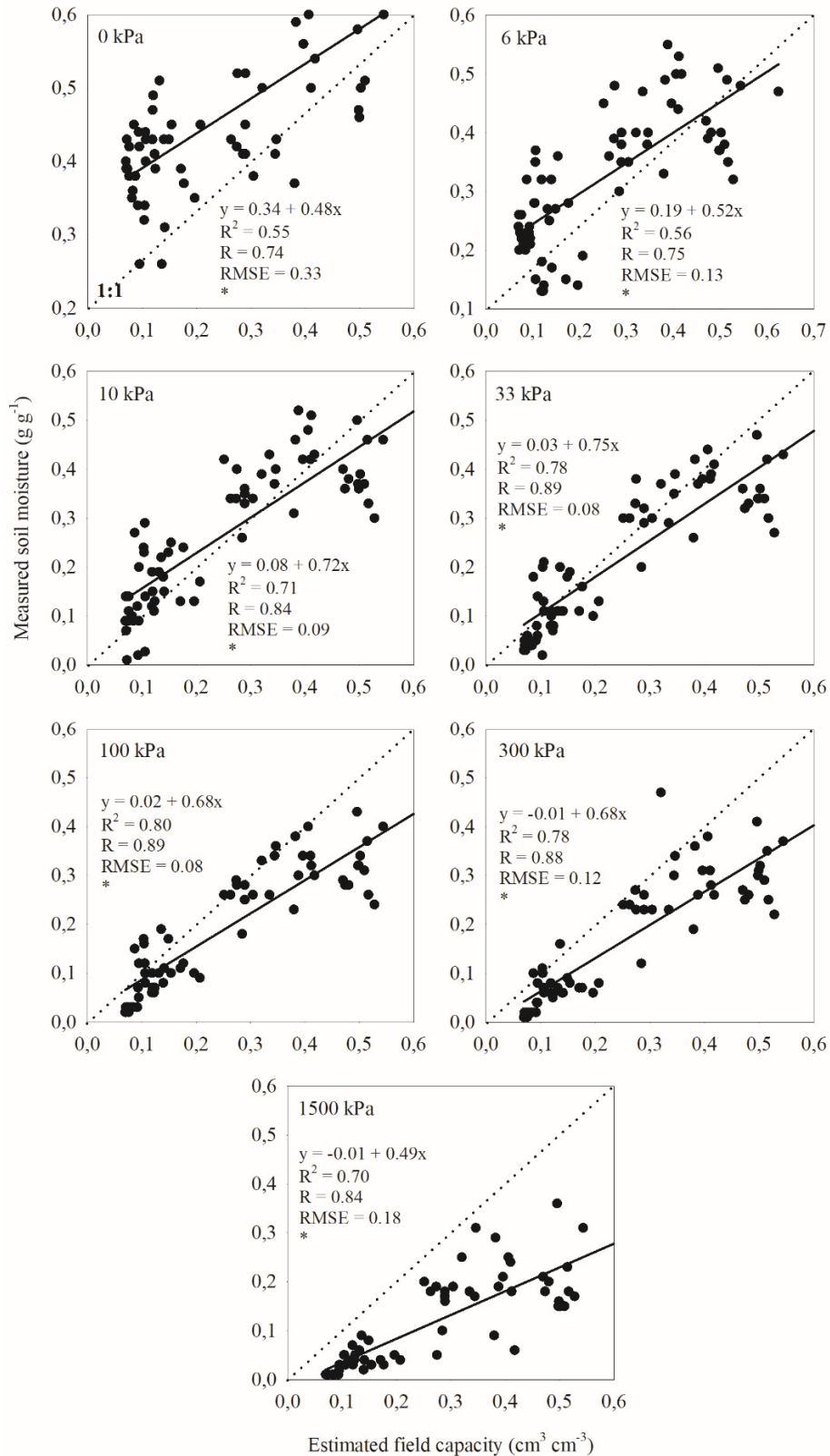
Figure 4. Linear regression between field capacity (FC) estimated using PTF-2 and soil moisture quantified at different tensions: 0, 6, 10, 33, 100, 300, and 1500(KPa). The dotted line represents the 1:1 regression line. *p<0.001 (F test).
