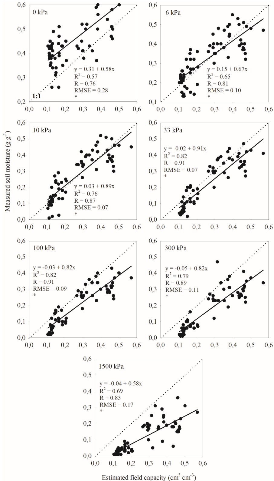
Figure 3. Linear regression between field capacity (FC) estimated by PTF-1 and soil moisture measured at different tensions (0, 6, 10, 33, 100, 300, and 1500 KPa). The dotted line represents the 1:1 regression line. * p < 0.001 (F test).
