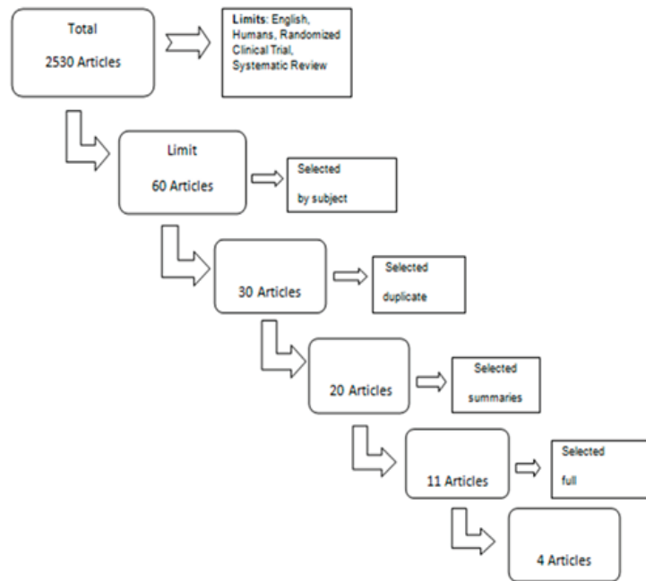
Figure 1 - Study flowchart
