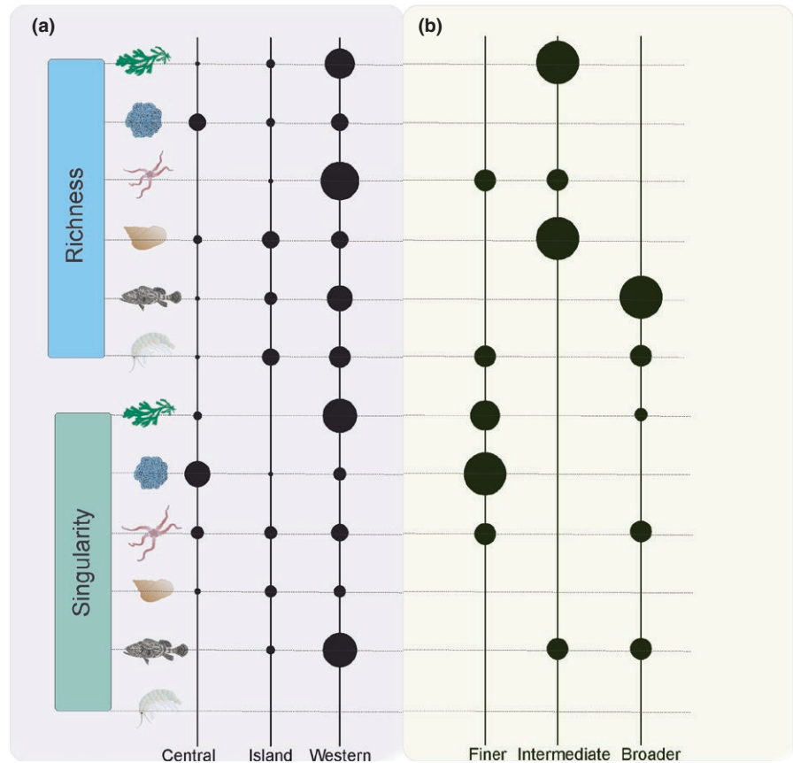
FIGURE 4 Patterns of richness and singularity of six taxonomic groups (from top to bottom: algae, corals, echinoderms, molluscs, fish, crustaceans) from 42 sites in Ilha Grande Bay, by (a) geographical location where symbol sizes represent proportion of the top 10 richest/most singular sites falling in each region and (b) spatial scale where symbols sizes represent proportion of selected PCNMs at each spatial scale
