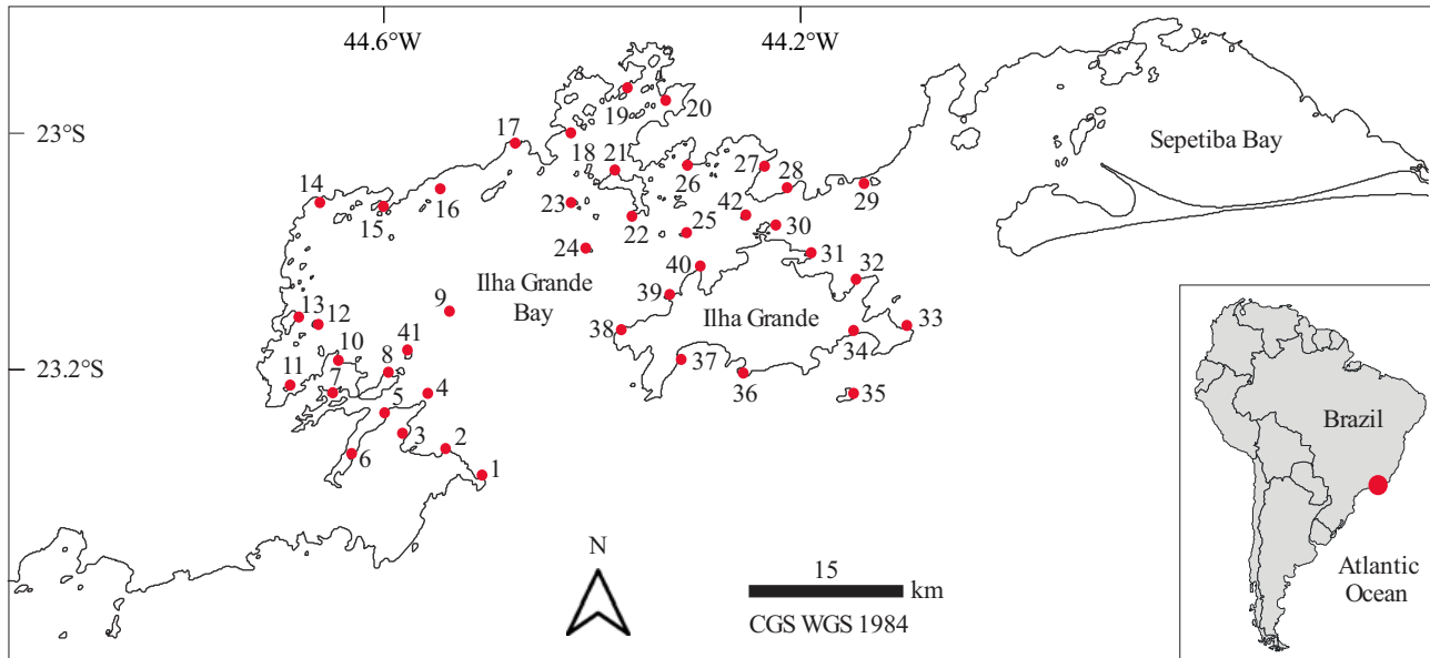
FIGURE 1 The 42 sampled sites (red dots) at Ilha Grande Bay, southeastern Brazil, as highlighted in the bottom right corner
