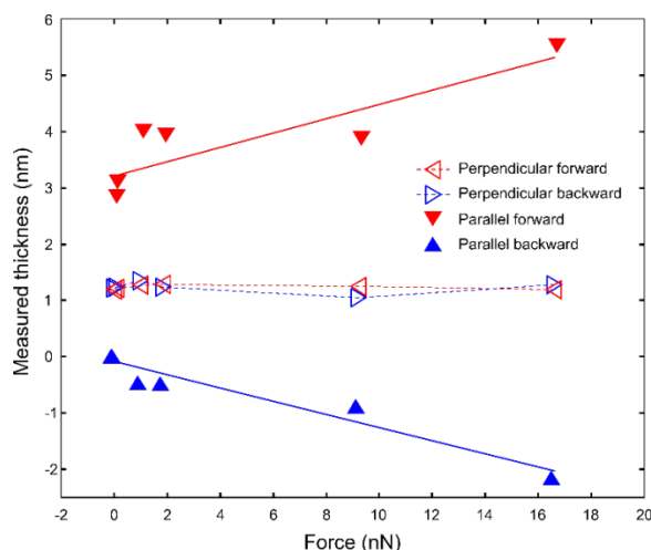
Figure 3. Experimental data of the apparent thickness of monolayer graphene as a function of the setpoint force for four different scan directions: Forward and Backward scanning directions for both perpendicular and parallel to the cantilever axis directions. The red and blue solid lines consist of a linear fit of the data, yielding h = 3.21 + 0.13F and h = -0.088 - 0.12F , respectively, where h is the apparent graphene thickness and F is the setpoint force.
