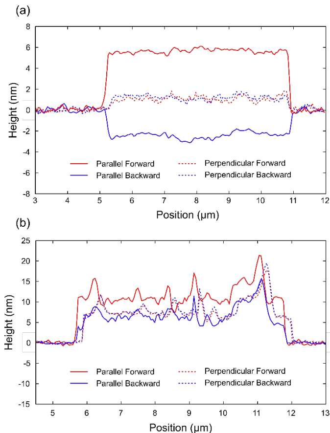
Figure 2. Line-scan profiles taken along the dotted lines in Fig. 1. Figure (a) shows the observed line profiles for graphene, while figure (b) shows line profiles for h-BN. The full lines (parallel scans) show the topographic artifact (graphene and h-BN thickness variation), whereas the dotted lines (perpendicular scans) indicate the correct topography.
