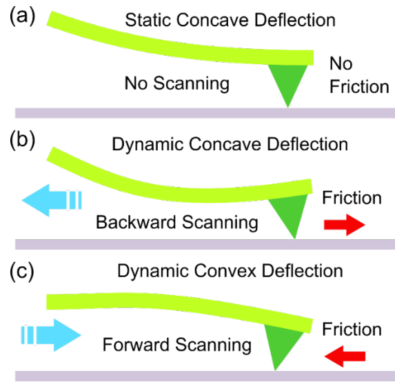
Figure 4. Qualitative picture of the topographic artifact. In (a), the cantilever is lowered to the surface while in a static situation (no scanning). Figure (b) shows a scan in the backward direction (to the left – blue arrow), where the friction force is in the opposite direction (to the right – red arrow). Figure (c) shows a scan in the forward direction (to the right) and the friction force is to the left. In figure (b), the cantilever bending is more pronounced (concave) than in (a), while in (c) it is less bent (convex) than in (a).
