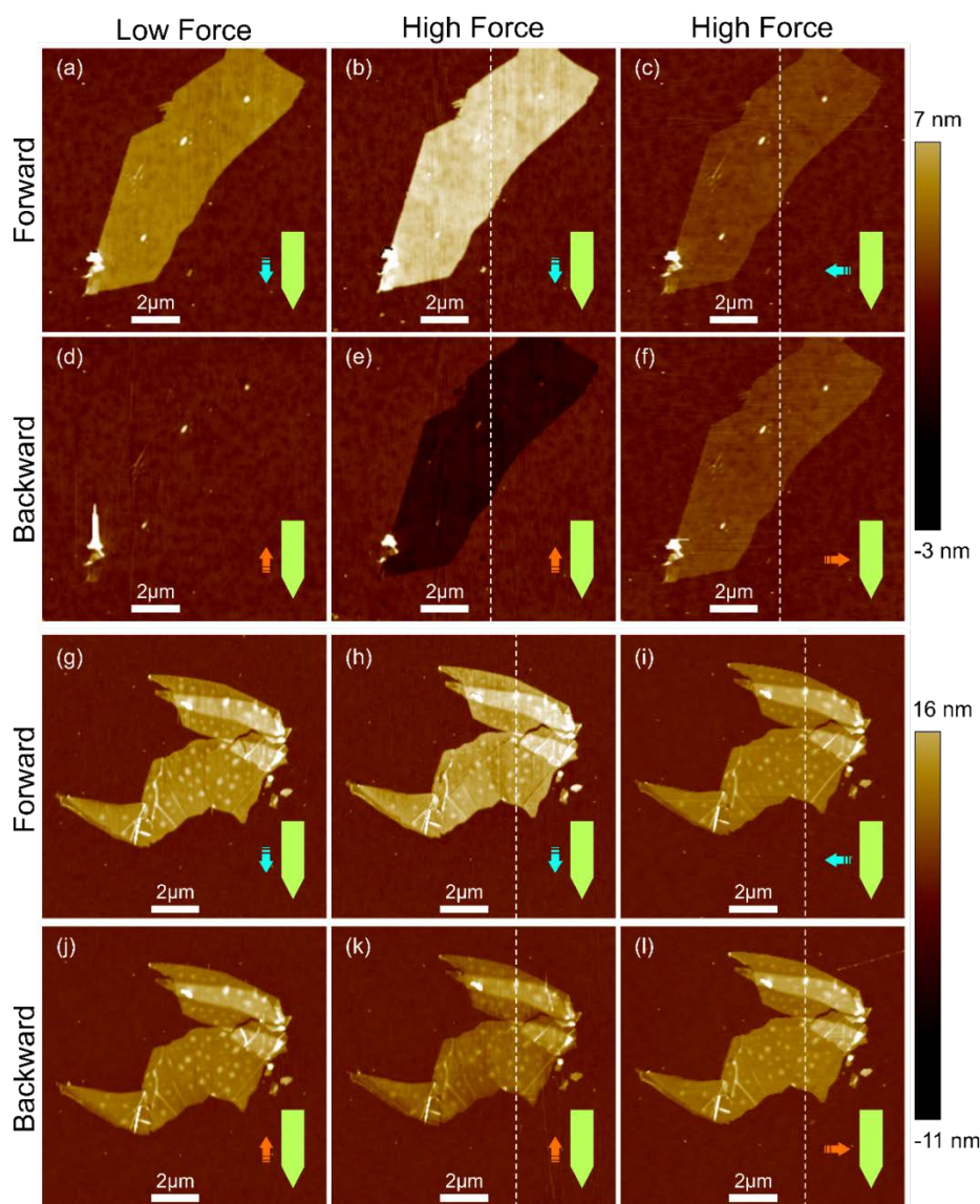
Figure 1. Topographic images of a monolayer graphene (a-f) and h-BN few-layer flake (g-l). The first column of images (Figures a, d, g and j) represents a low-force regime for the parallel geometry, the second column (Figures b, e, h and k) constitutes a high-force regime for the parallel geometry and the third column (Figures c, f, i and l) represent a high-force regime for the perpendicular geometry. The definition of Forward and Backward scanning directions is shown in the insets at the bottom right of each image, where the green symbol depicts the AFM cantilever and the red and cyan arrows indicate the scanning orientation.
