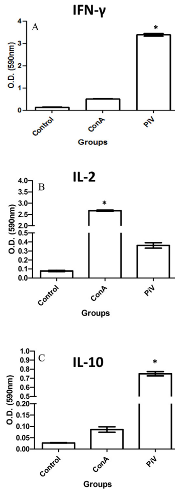
Fig. 4. ELISA analysis of cytokines from the control group and the PiV- and Leishmania major -challenged mice. This figure shows that the control group, challenged only with L. major , exhibited significant differences in cytokine production compared with mice challenged with both PiV and L. major . The expression of IFN- \gamma (ELISA) in the supernatant of mouse splenic cells after 72 h of stimulation with PiV (OD 3.3 = 660 pg/ml) or Concanavalin A (ConA) (OD 0.4 = 111 pg/ml) is shown in Panel A. The graph in panel A displays contrasting differences with the control group challenged with L. major only (undetectable levels, below sensitivity of the test). Panel B depicts expression of IL-2 (ELISA) in the supernatant of mouse splenic cells stimulated with PiV (OD 0.39 = 150 pg/ml) or with ConA (OD 2.7 = 1000 pg/ml) after 72 h of stimulation. This panel also shows significant differences with the control group challenged only with L. major (OD 0.09 = 15 pg/ml). Panel C shows the expression of IL-10 in ELISA of splenocytes in PiV-immunized, L. major challenged BALB/c mice after 72 h of stimulation with PiV (OD 0.79 = 450 pg/ml) or ConA (OD 0.10 = 50 pg/ml). IL-10 detection in non-immunized mice was low (OD 0.03 = 15 pg/ml).
