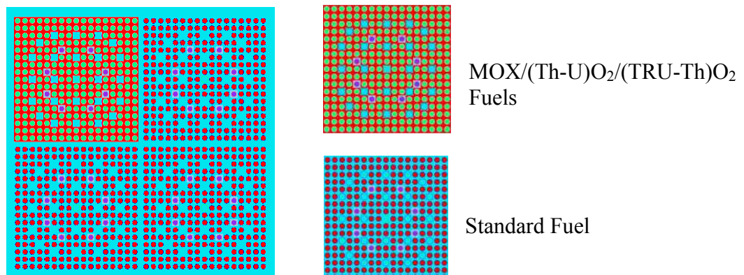
Figure 5: 1:3 ratio configuration for SFP using MOX, (Th-U)O_2 or (TRU-Th)O_2 with standard UO_2 fuel.
