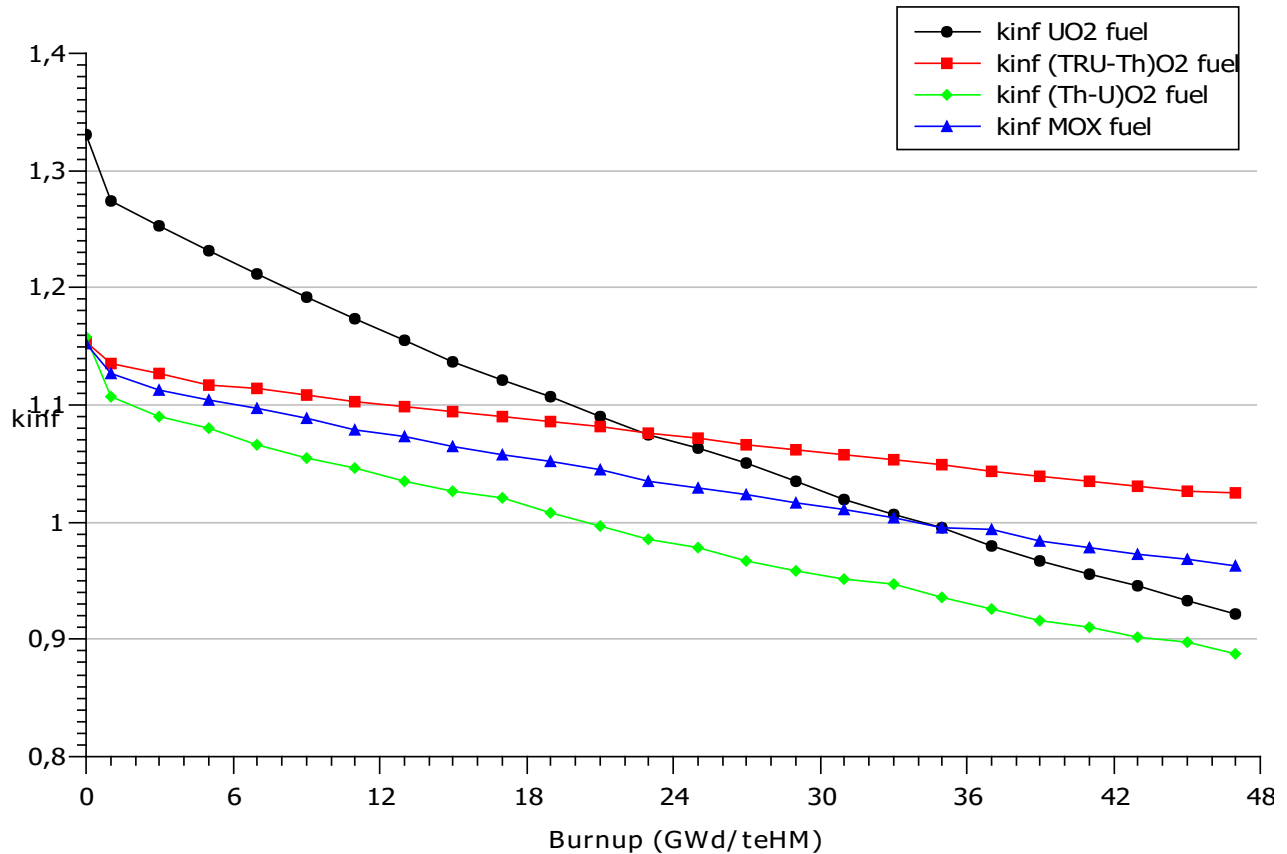
Figure 3: k_{inf} considering the 3 cycles for a single assembly irradiated in PWR reactor.
