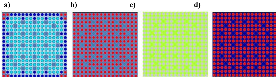
Figure 2: Fuel elements geometry adopted for Spent Fuel Pool criticality analysis. a) MOX, b) (Th-U)O 2 , c) (TRU-Th)O 2 and d) UO 2 .
