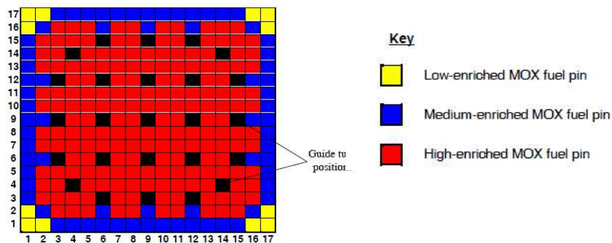
Figure 1: MOX fuel assembly [8].
