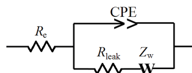
Fig. 7 – Randles equivalent circuit used to fit impedance data
