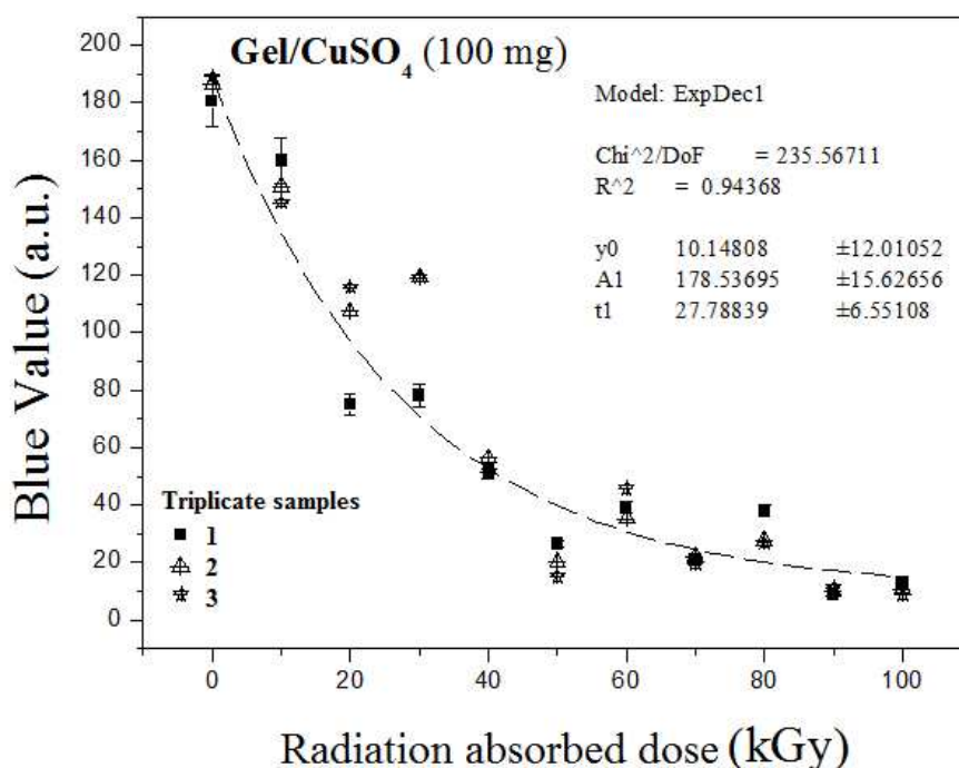
Figure 2: Variation of blue values as a function of absorbed dose of the gel/ \text{CuSO}_4 (100 mg) no irradiated and gamma irradiated with doses between 10 – 100 kGy.
