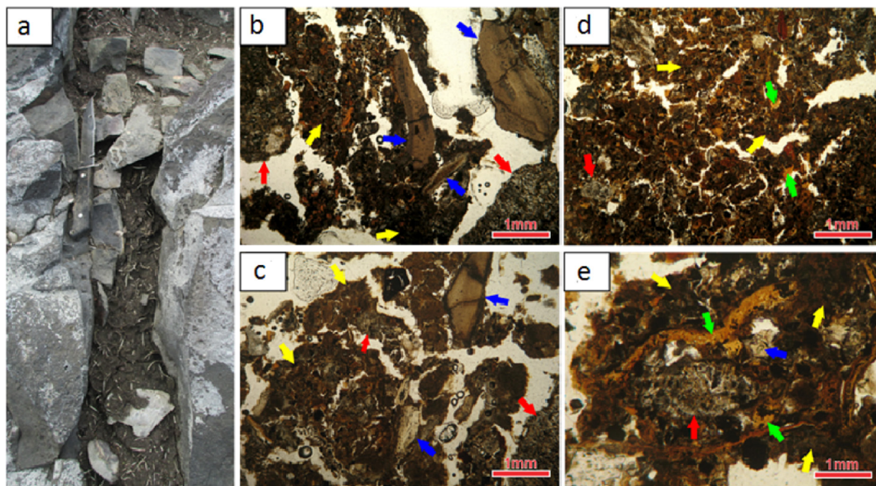
Figure 5. a) Macromorphological aspect and b, c, d, e) Micromorphological representative photomicrographs in ppl (parallel polarized light) of soil pockets affected by flying birds (phosphatized soils). Blue arrows indicate bone fragments. Red arrows indicate rock fragments. Yellow arrows indicate phosphatized micromass. Green arrows indicate amorphous iluvial Fe-P features.
