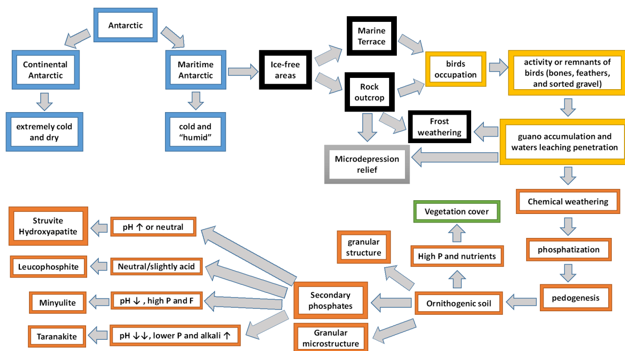
Figure 6. Integrated scheme of ornithogenic soil formation in Maritime Antarctica, the mineral assemblage representative of phosphatization and pedoenvironmental features. Blue color indicates association with climate conditions, black association with lithology, gray association with relief, yellow association with faunal activities, orange association with soil and green association with plants. Based on Tatur & Myrcha (1984), Simas et al. (2007), Schaefer et al. (2008) and Pereira et al. (2013).
