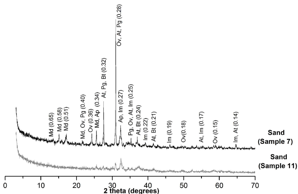
Figure 2. Representative XRD of sand samples of ornithogenic sites (samples 7 and 11).
