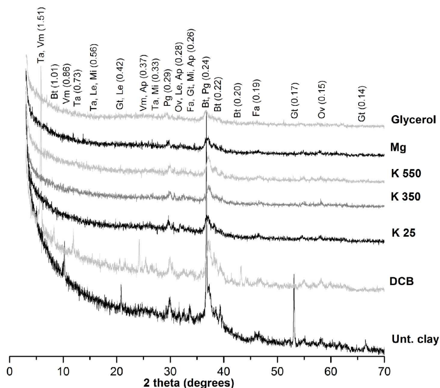
Figure 4. Representative XRD of clay sample of ornithogenic soil (sample 11). Unt. Clay - Untreated clay; DCB - removal of iron oxides; K - K + saturation (heat treatment of K-saturated mounts to 25°, 350° and 550° C); Mg - Mg 2+ saturation; Glycerol - saturated by Mg 2+ and solvated by glycerol. Vm - vermiculite; Bt - biotite; Pg - plagioclase; Le - leucophosphite; Mi - minyulite; Gt - goethite; Fa - fluorapatite; Ov - olivine; Ap - apatite; Ta - taranakite. "d" in nm.
