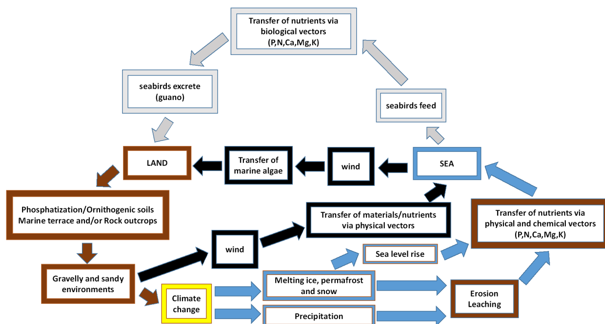
Figure 7. A proposal model of sea-land nutrient transfer in Maritime Antarctica, using climate change scenario, biological, physical and chemical vectors. Blue color indicates association with water, black association wind, gray association with seabirds, yellow association with climate and brown association with land. Informations extraction from Simas et al. (2007), Qin et al. (2014), Schaefer et al. (2017) and Otero et al. (2018).
