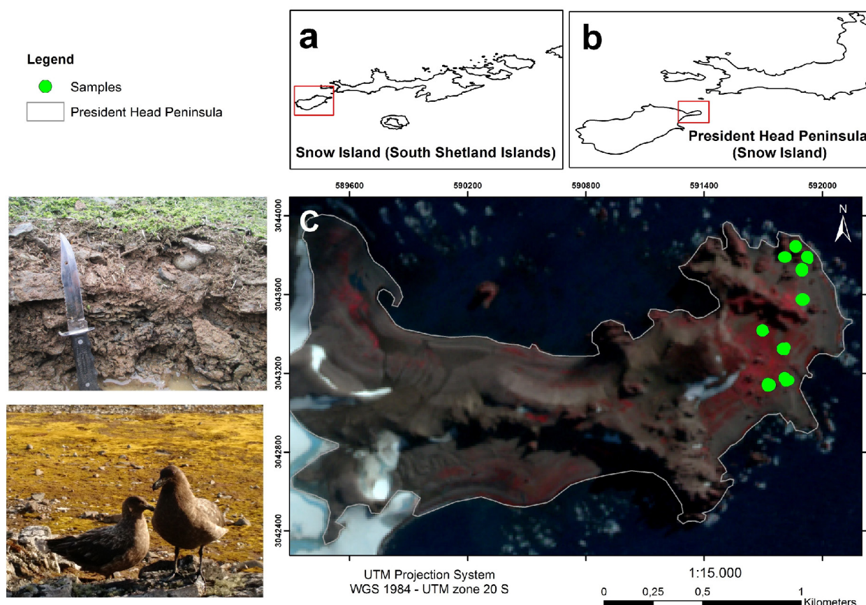
Figure 1. Localization of President Head Peninsula (c), Snow Island (b), South Shetlands Islands (a).
