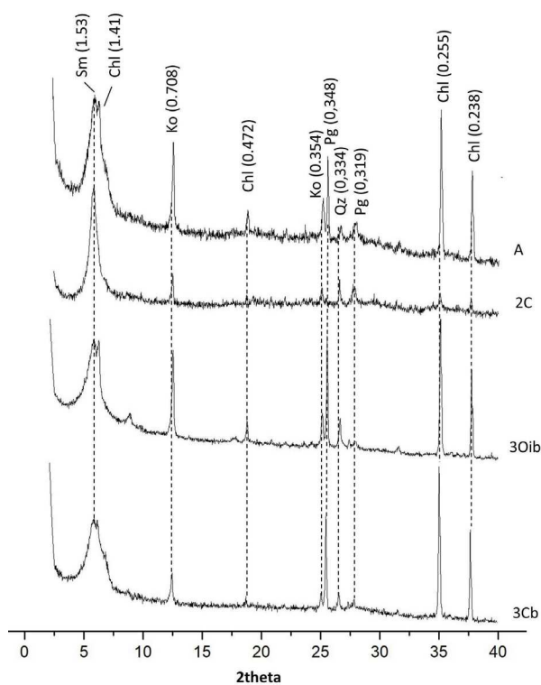
Figure 3. XRD spectrum of clay fraction within the pedon P2 (MT-1). Chl: chlorite, Sm: smectite, Ko: kaolinite Pg: plagioclase, Qz: quartz. "d" in nm.
