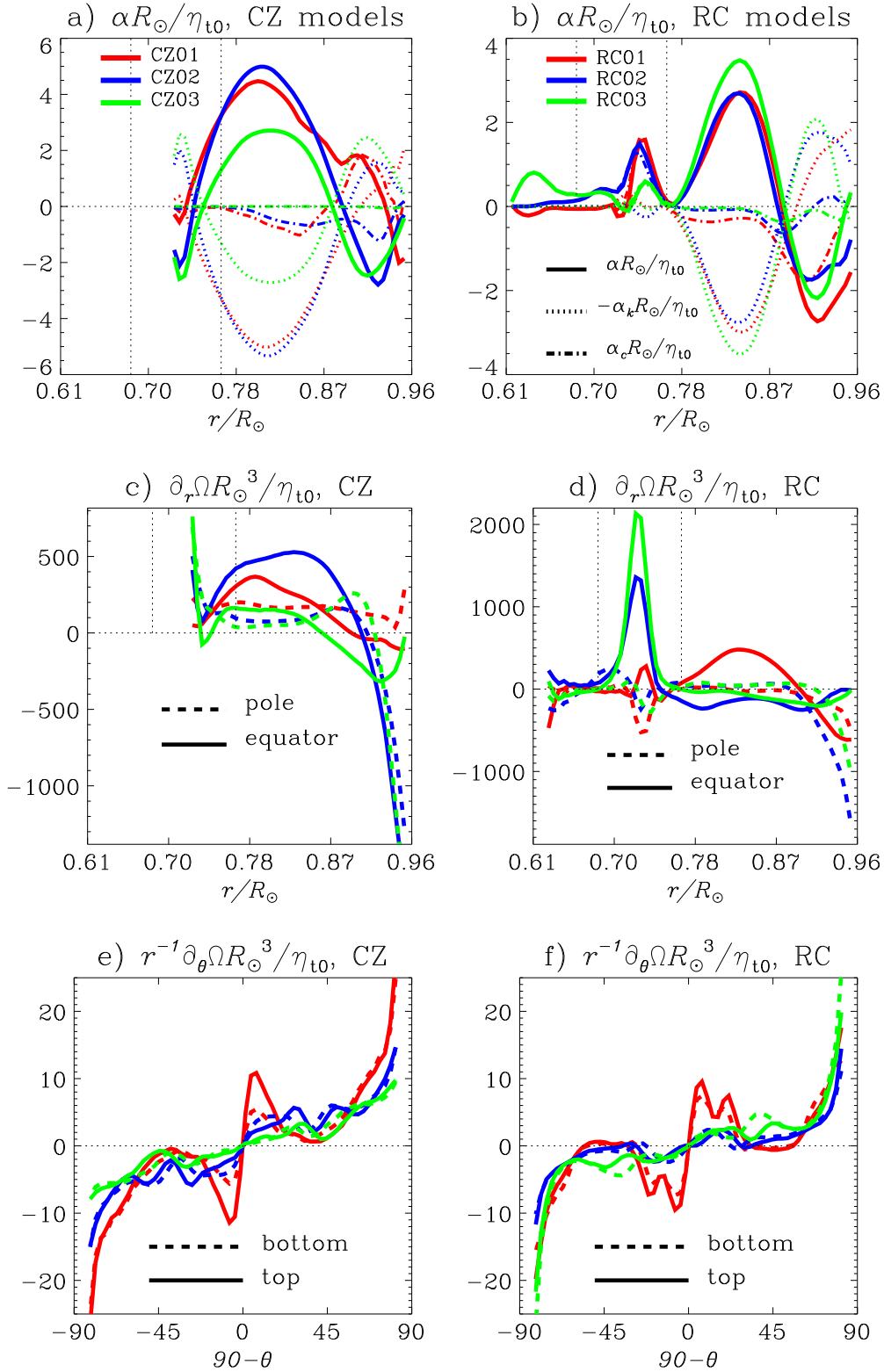
Figure 3. Magnetic field source terms (see Equations (8)–(9)) for models CZ (left panels) and RC (right). Panels (a) and (b) show the FOSA estimation for \alpha R_\odot/\eta_{t0} . Dotted and dotted–dashed lines represent the kinetic and magnetic contribution, respectively. The continuous line is the resultant, non-dimensional, total \alpha -effect. The profiles of \alpha are latitudinal averages in the northern hemisphere. Middle and bottom rows show \partial_r \Omega R_\odot^3/\eta_{t0} and r^{-1} \partial_\theta \Omega R_\odot^3/\eta_{t0} , respectively. In panels (c) and (d) continuous (dashed) lines indicate latitudinal averages at lower, 20^\circ – 40^\circ (higher, 60^\circ – 80^\circ ), latitudes. (Note that in panel (d) the value of \partial_r \Omega R_\odot^3/\eta_{t0} for the model RC03 has been divided by 2.) In panels (e) and (f) continuous (dashed) lines are vertical averages in the top, 0.9 R_\odot \leq r \leq 0.95 R_\odot (bottom, 0.72 R_\odot \leq r \leq 0.77 R_\odot ), of the domain. \eta_{t0} is a radial average of \eta_t , defined in Equation (9), for r \geq 0.72 R_\odot .
