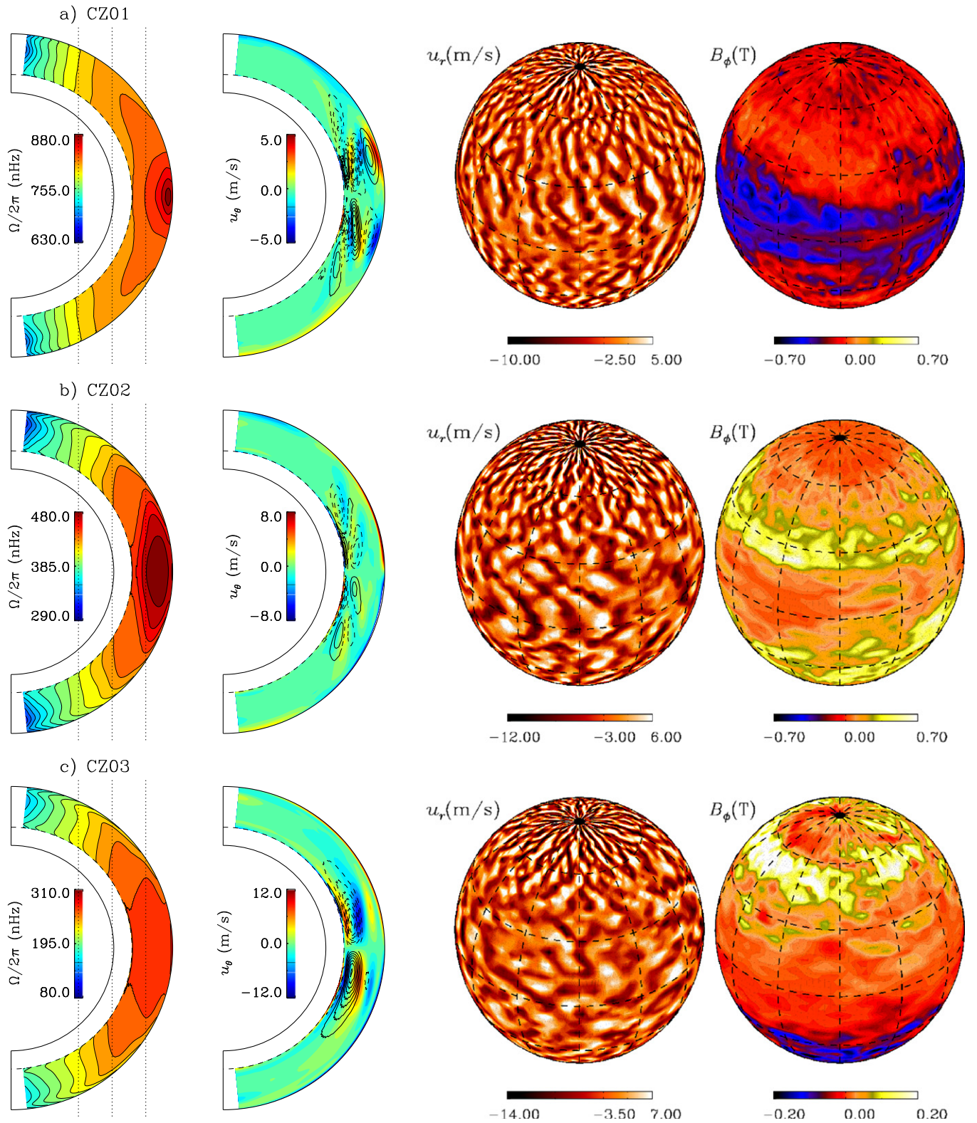
Figure 1. From left to right: mean profiles of the rotation rate and meridional circulation, and snapshots at r = 0.95R_\odot of the vertical velocity, u_r , and the toroidal field, B_\phi , for the simulated models (a) CZ01, (b) CZ02, and (c) CZ03. In the meridional circulation panels continuous (dashed) lines correspond to clockwise (counterclockwise) circulation. The background filled contours show the latitudinal velocity, \bar{u}_\theta . The profiles of differential rotation and meridional circulation correspond to mean azimuthal values averaged over \sim 3 yr during the steady-state phase of the simulation.
