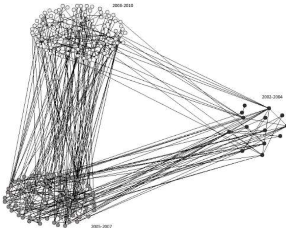
Figure 13 - Co-authorship network – Co-authorship relationships x length of time in the network
