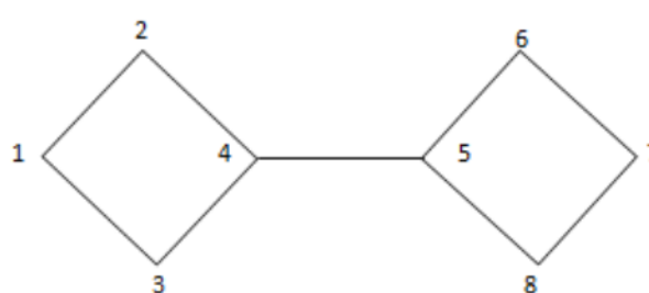
Figure 2 - Structural hole hypothesis Source: Klovdahl's graph (1992).
