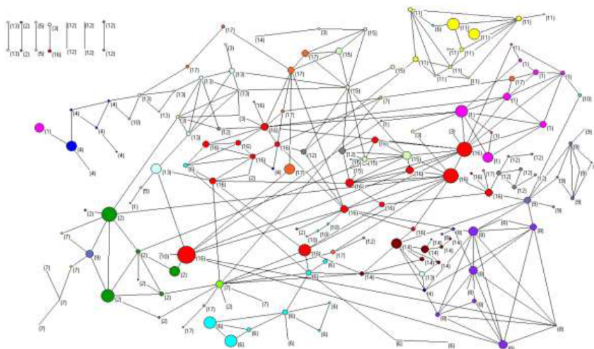
Figure 14 - Co-authorship network - Productivity x postgraduate programs
