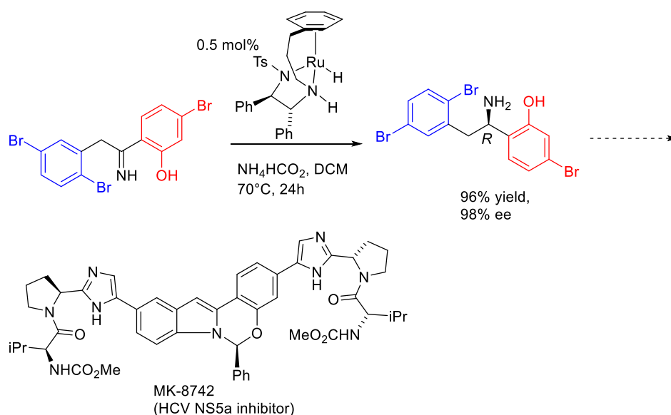
Figure 13. A reported imine ATH using a tethered catalyst.
