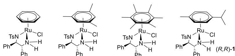
Figure 5. Variation of the \eta^6 -arene ring in Noyori–Ikariya catalysts.
