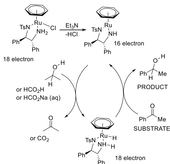
Figure 2. Mechanism of hydrogen transfer with Noyori–Ikariya catalysts.
