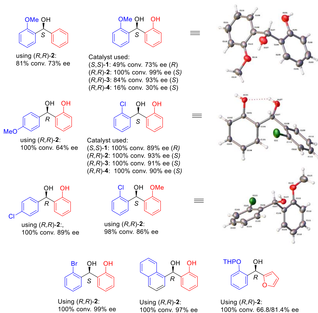
Figure 10. Further examples of ATH of ortho -hydroxy benzophenones.
