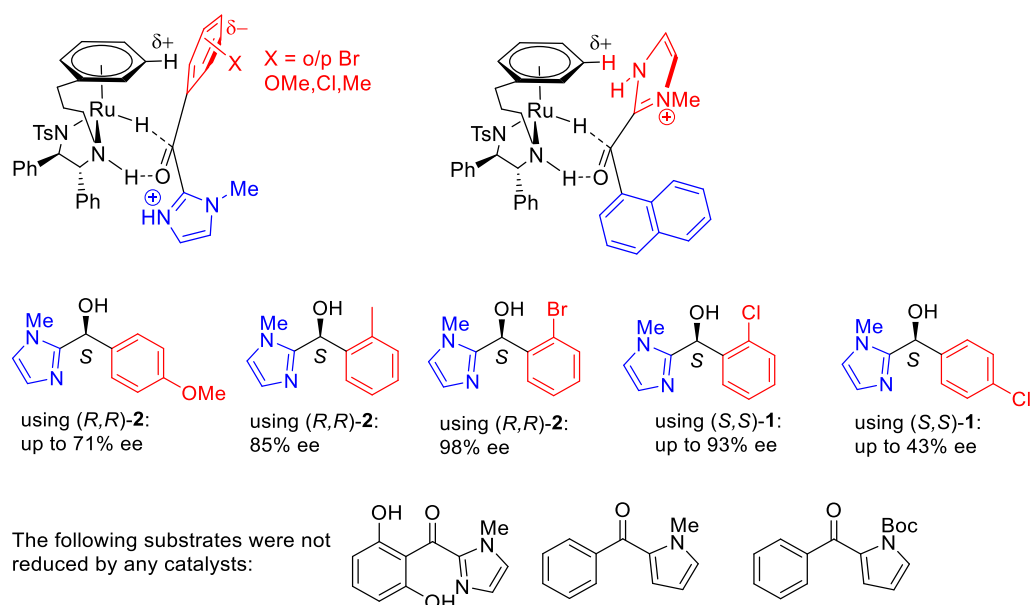
Figure 19. Products of ATH of an extended range of aromatic/heterocyclic ketones, and proposed modes of hydrogen transfer to substrates.
