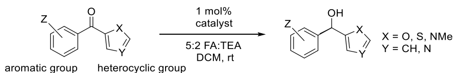
Figure 16. ATH of heterocyclic/aromatic ketones—reported examples.
