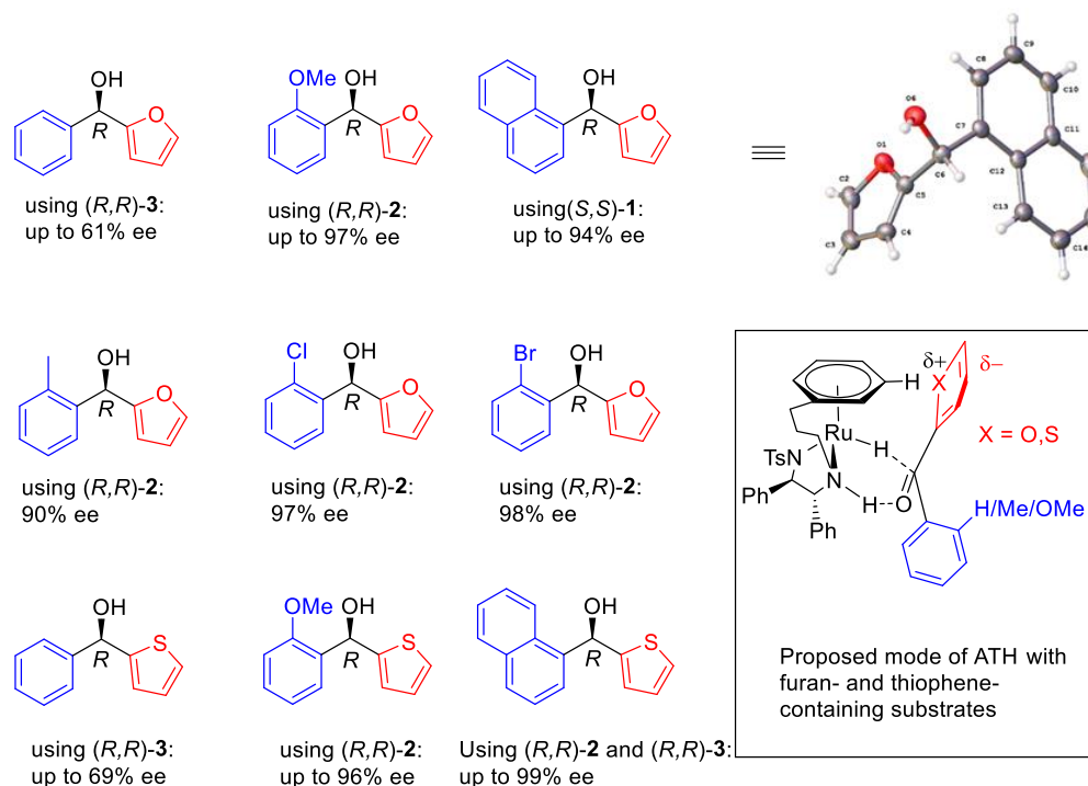
Figure 17. ATH of aromatic/heterocyclic ketones in this product.
