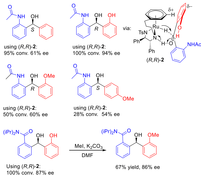
Figure 12. ATH of benzophenones containing amides.
