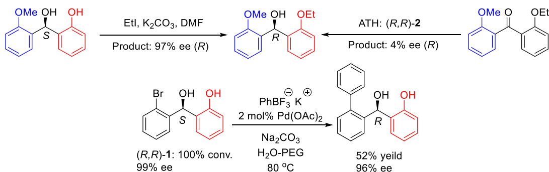
Figure 15. Functionalizations of the ATH products.
