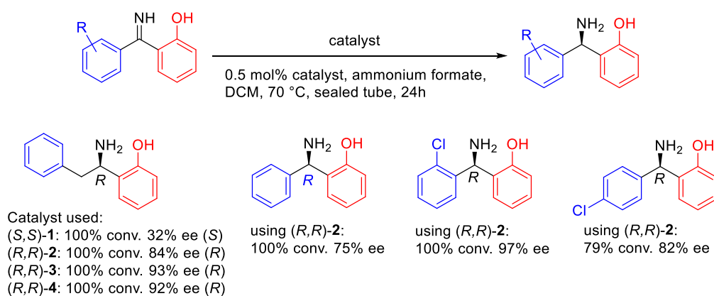
Figure 14. ATH of imines using a tethered catalyst.
