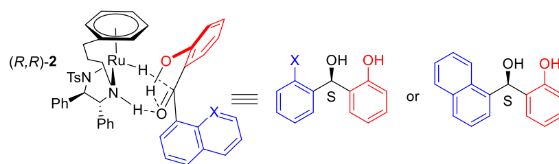
Figure 11. Involvement of H-bond in reduction mechanism.
