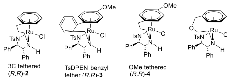
Figure 6. Tethered catalysts introduced by Wills et al.
