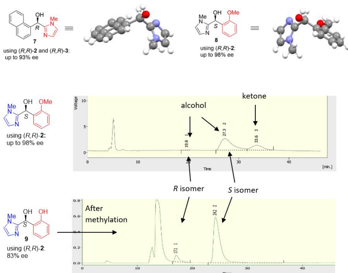
Figure 18. Determination of configuration of ATH products containing imidazole groups.
