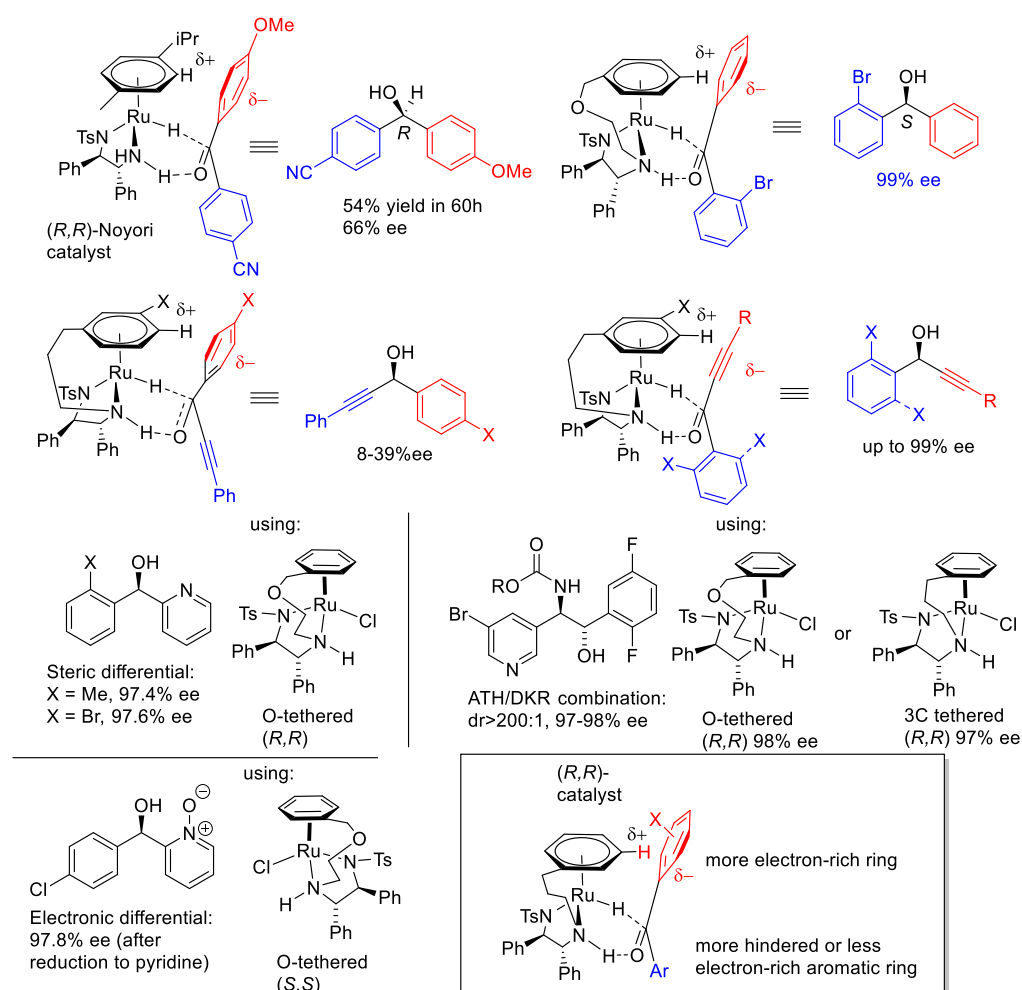
Figure 7. Examples of ATH of benzophenone derivatives and heterocyclic ketones using Noyori-Ikariya catalysts (The red part favours positioning adjacent to \eta^6 -arene of catalyst, while the blue part favours positioning distal to \eta^6 -arene of catalyst).
