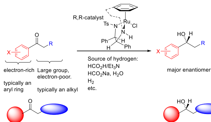
Figure 4. Summary of stereocontrol features in ATH using Noyori–Ikariya catalysts.
