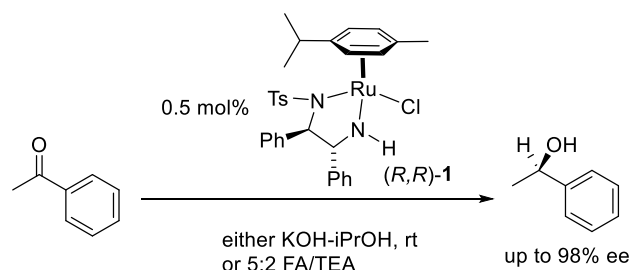
Figure 1. Asymmetric Transfer Hydrogenation (ATH) with Noyori-Ikariya catalysts.
