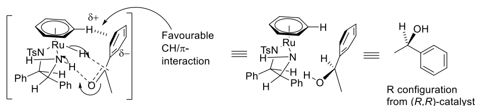
Figure 3. Interaction of substrate with \eta^6 -arene ring.
