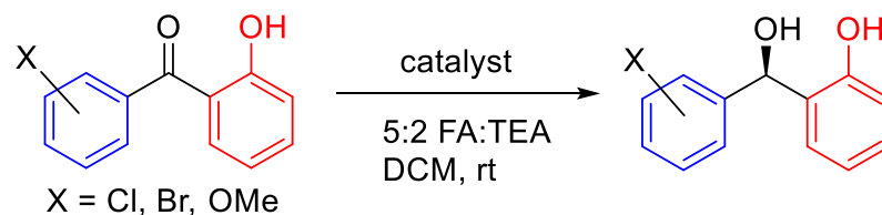
Figure 8. ATH of ortho -hydroxy benzophenones using tethered ATH complexes.
