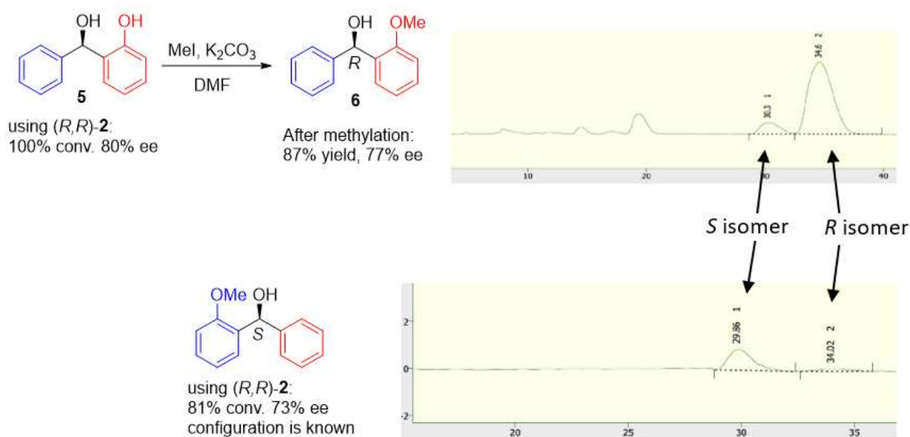
Figure 9. Determination of product configuration in ATH of ortho -hydroxy benzophenones.
