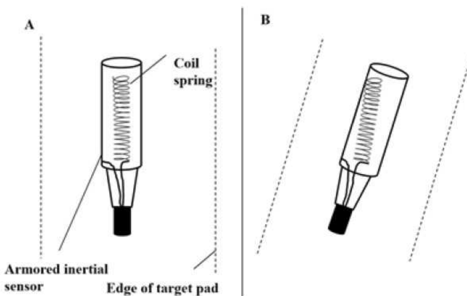
Figure 2. Coupled inertial sensor inside the target pad: (A) – before the kick contact; (B) – after the kick contact (closed electronic circuit between the coil spring and the armoured inertial sensor).
