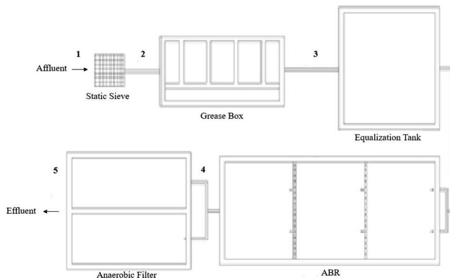
Figure 1. Schematic drawing of the wastewater treatment system.
