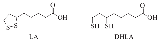
Figure 2. Chemical structures of lipoic acid (LA) and of dihydrolipoic acid (DHLA).
