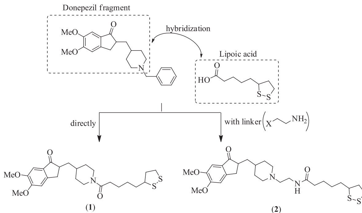
Figure 3. Design strategy for hybrids 1 and 2 .
