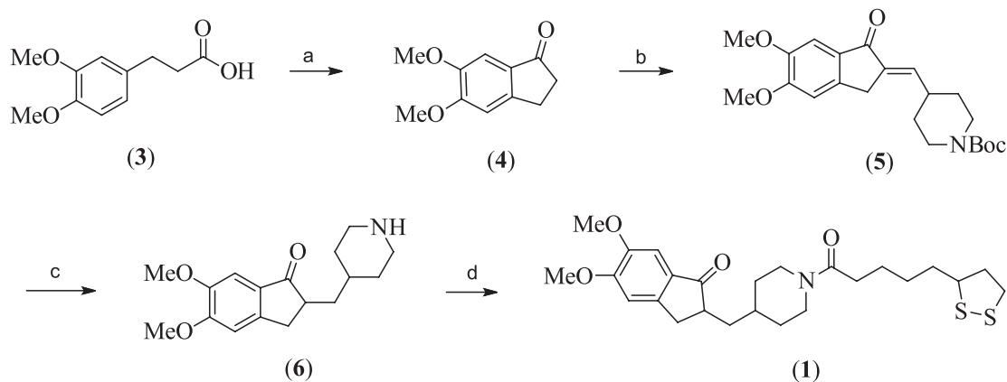
Scheme 1. Synthesis of donepezil-LA hybrid 1 . Reagents and conditions: (a) p -toluenesulfonic acid, P 2 O 5 , 120 °C, 35 min, 87%; (b) N -Boc-piperidine-4-carboxaldehyde, NaH, tetrahydrofuran (THF), r.t., 2 h, 84%; (c) H 2 (1 atm), Pd-C (10%), THF, r.t., 20 min, then hydrochloric acid (HCl) (3 M), ethyl acetate (EtOAc), r.t., 3 h, 91%; (d) lipoic acid, DIPEA, PyBOP, dichloromethane (DCM), 0 °C → r.t., 20 h, 63%.
