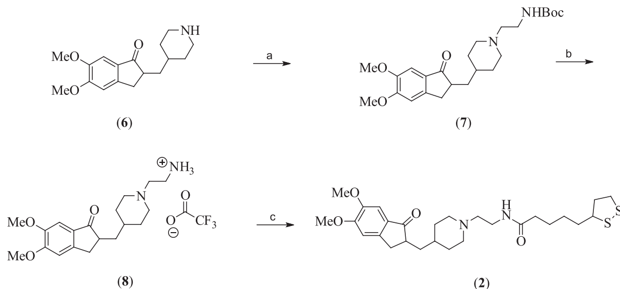
Scheme 2. Synthesis of donepezil-LA hybrid 2 . Reagents and conditions: (a) tert -butyl (2-bromoethyl)carbamate, DIPEA, sodium iodide (NaI), acetonitrile (MeCN), reflux, 24 h, 39%; (b) TFA, DCM, r.t., 1 h, 100%; (c) lipoic acid, DIPEA, PyBOP, DCM, 0 °C → r.t., 20 h, 74%.
