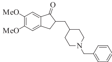
Figure 1. Chemical structure of donepezil.
