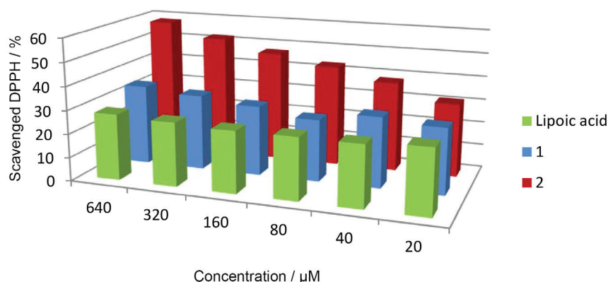
Figure 4. Antioxidant activity toward DPPH radicals expressed as percentage.
