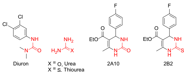
Fig. 1. Structure of urea and thiourea analogues evaluated for the ability to impair weed growth. Urea and thiourea moieties are highlighted in red color.
