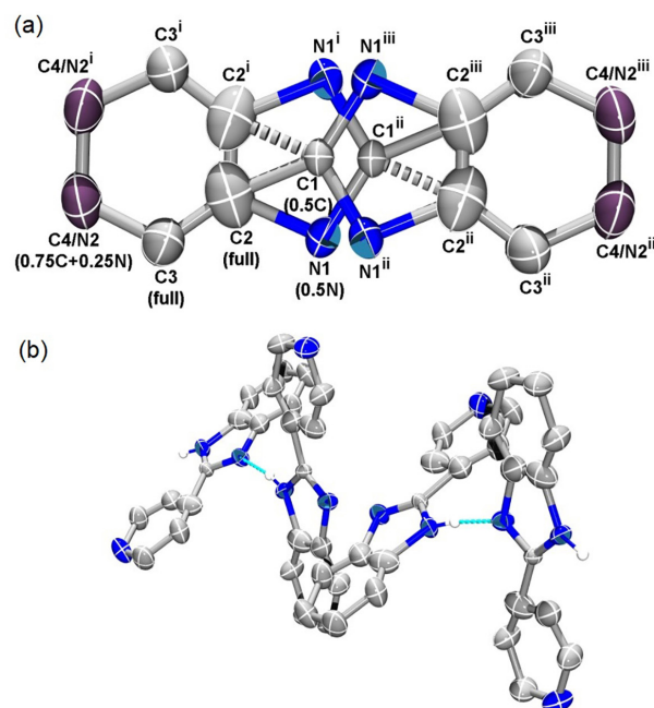
Figure 2. (a) 30% ellipsoid plot of the BIA molecule disordered over two occupancy site sets, whose benzene and pyridyl rings were found to be overlaid in this study. (b) One possible hydrogen bonding array in the crystal packing of BIA is determined here, with imidazole NH hydrogens covalently bonded to four imidazole nitrogen atoms equivalent to the four shown in (a).
