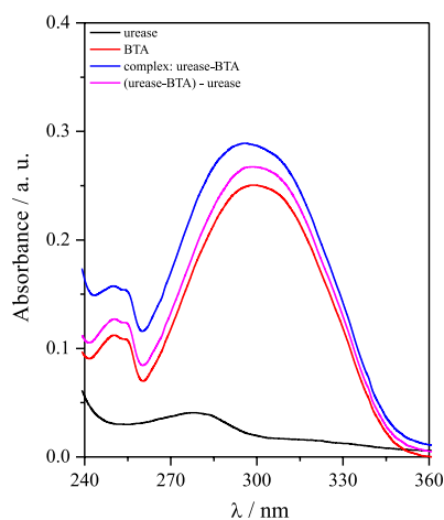
Figure 5. UV-Vis absorption spectra of urease (3 \mu\text{M} ), BTA (15 \mu\text{M} ), urease-BTA complex, and (urease-BTA) - urease at pH 7.4 and 28 °C.
