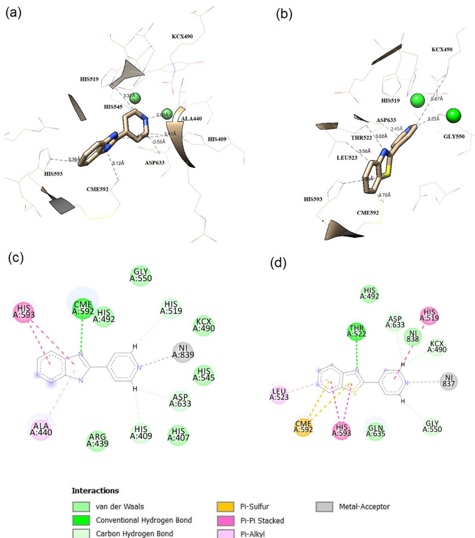
Figure 8. (a) BIA and (b) BTA interactions with Ni metals and residues from the jack bean urease. The binding conformation of the ligands are shown in stick representation, and green spheres represent the two Ni metals. Coordination with Ni metals, hydrogen bonding, \pi - \pi stacking, \pi -alkyl, \pi -sulfur, and van der Waals interactions are shown as dotted lines. (c, d) 2D-interaction diagram of BIA and BTA, respectively.
