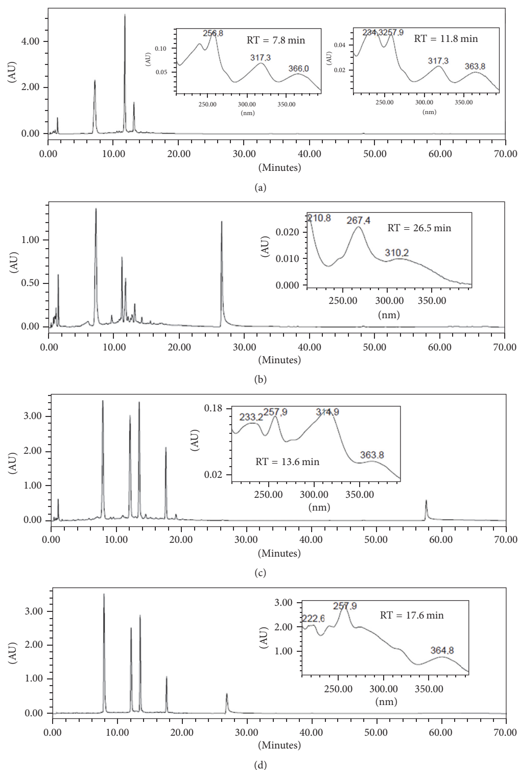
FIGURE 1: RP-HPLC-DAD fingerprints for the crude ethanol extracts from (a) ethanol extract from Fridericia formosa leaves (EEFLL) with mangiferin (RT = 7.8 min) and 2'-O-trans-caffeoylmangiferin (RT = 11.8 min) UV spectrum registered online detection 350 nm, (b) ethanol extract from Fridericia formosa stems (EEFFS) with UV spectra registered online for peak corresponding to chrysin (RT = 26.8 min), (c) ethanol extract from Fridericia formosa fruits (EEFFF) with UV spectra registered online for peak corresponding to 2'-O-trans-coumaroylmangiferin (RT = 13.6 min), and (d) for a mixture of the isolated compounds with UV spectra registered online for peak corresponding to 2'-O-trans-cinnamoylmangiferin (RT = 17.6 min). Detection: 350 nm. Chromatographic conditions: see Experimental.
