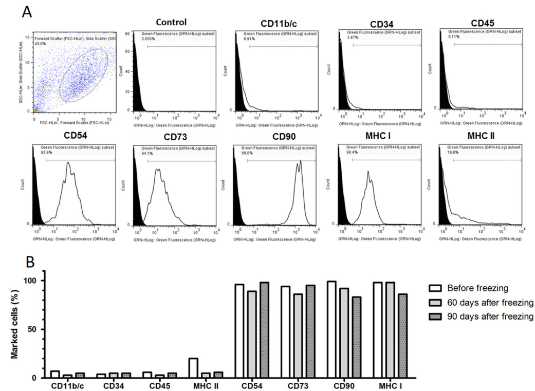
Figure 1. A. Histograms of the expression of CD11, CD34, CD45, CD54, CD73, CD90, MHC I, and MHC II by flow cytometry in cultures of MSCs of rat adipose tissue. The white graph represents the population of cells evaluated for a specific marker (offset to the right indicates the existence of staining). B. Percentage of cells expressing the markers CD11, CD34, CD45, CD54, CD73, CD90, MHC I, and MHC II before freezing and 60 and 90 days after freezing.
