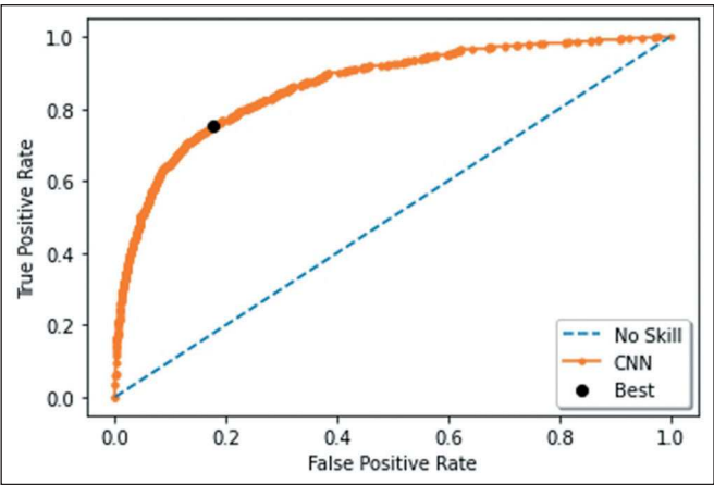
Figure 4. Receiver operating characteristic curve for the model. The black dot demonstrates the threshold of highest balanced accuracy.
