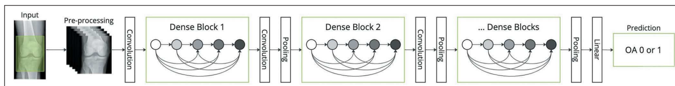
Figure 2. Schematic illustration of the DenseNet architecture. Pairs of layers are connected, allowing elements from the first layers (such as edges) to be used in the subsequent layers as well. Adapted from Huang et al. (20) .
